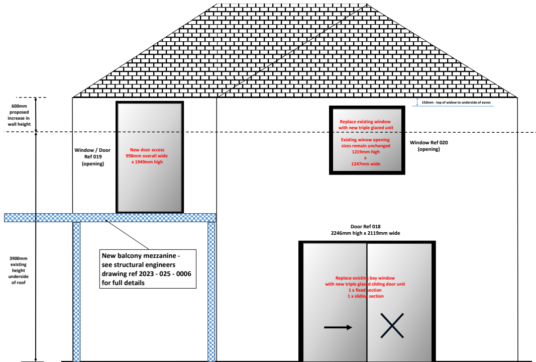
South Elevation - Proposed
