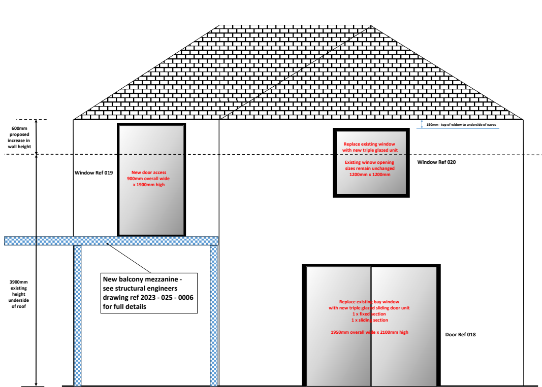
South Elevation - Proposed
