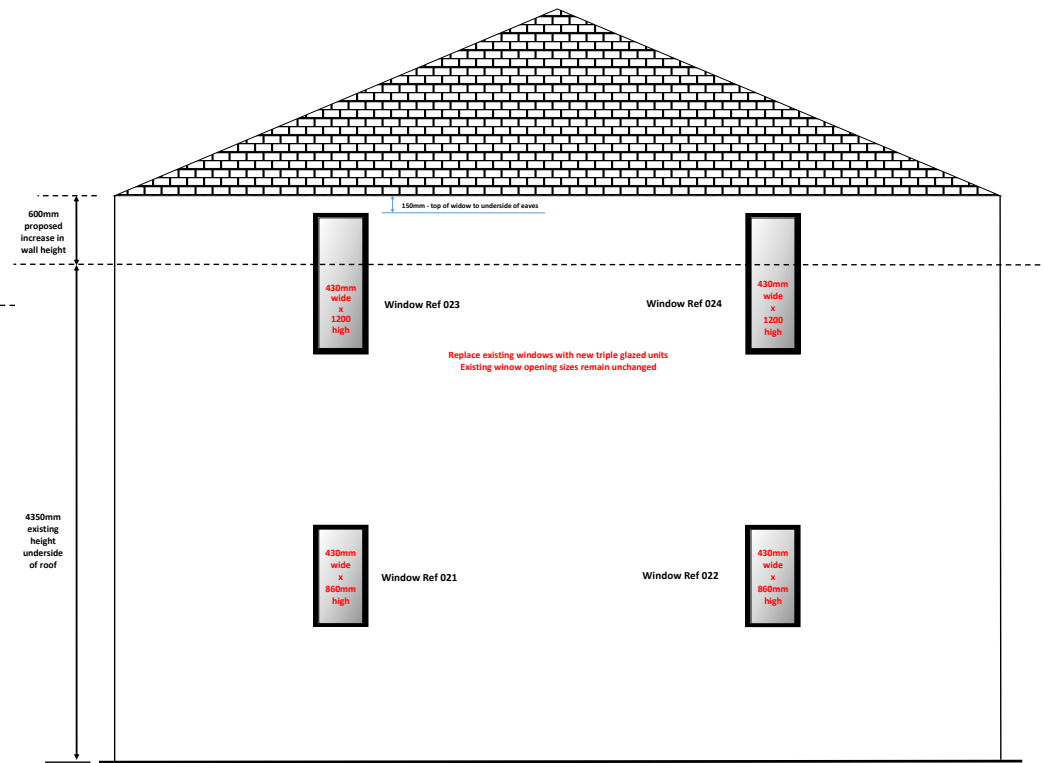
North Elevation - Proposed
