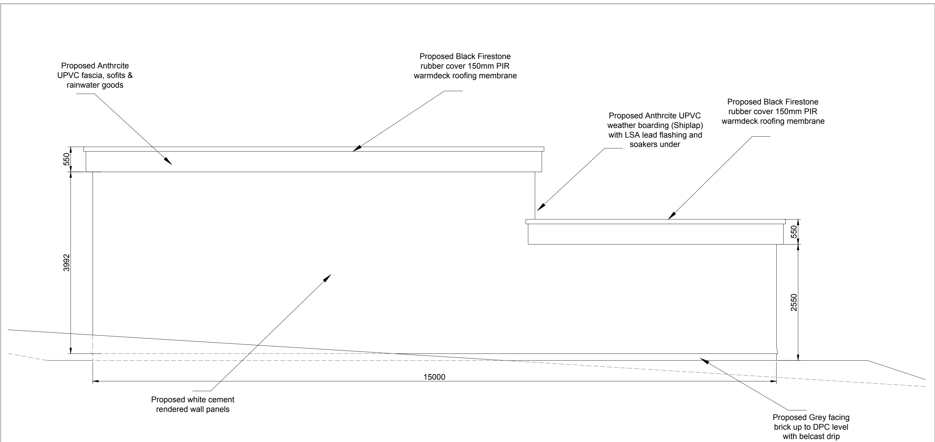
East Elevation
