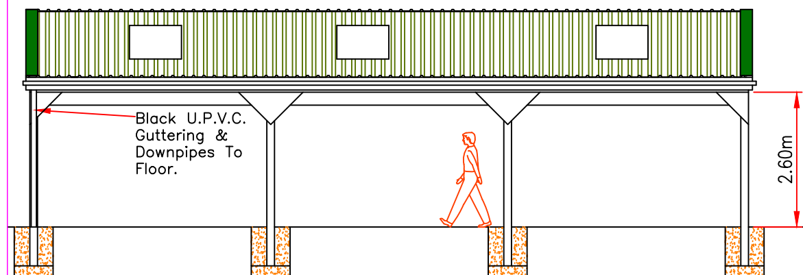
Rear Elevation
