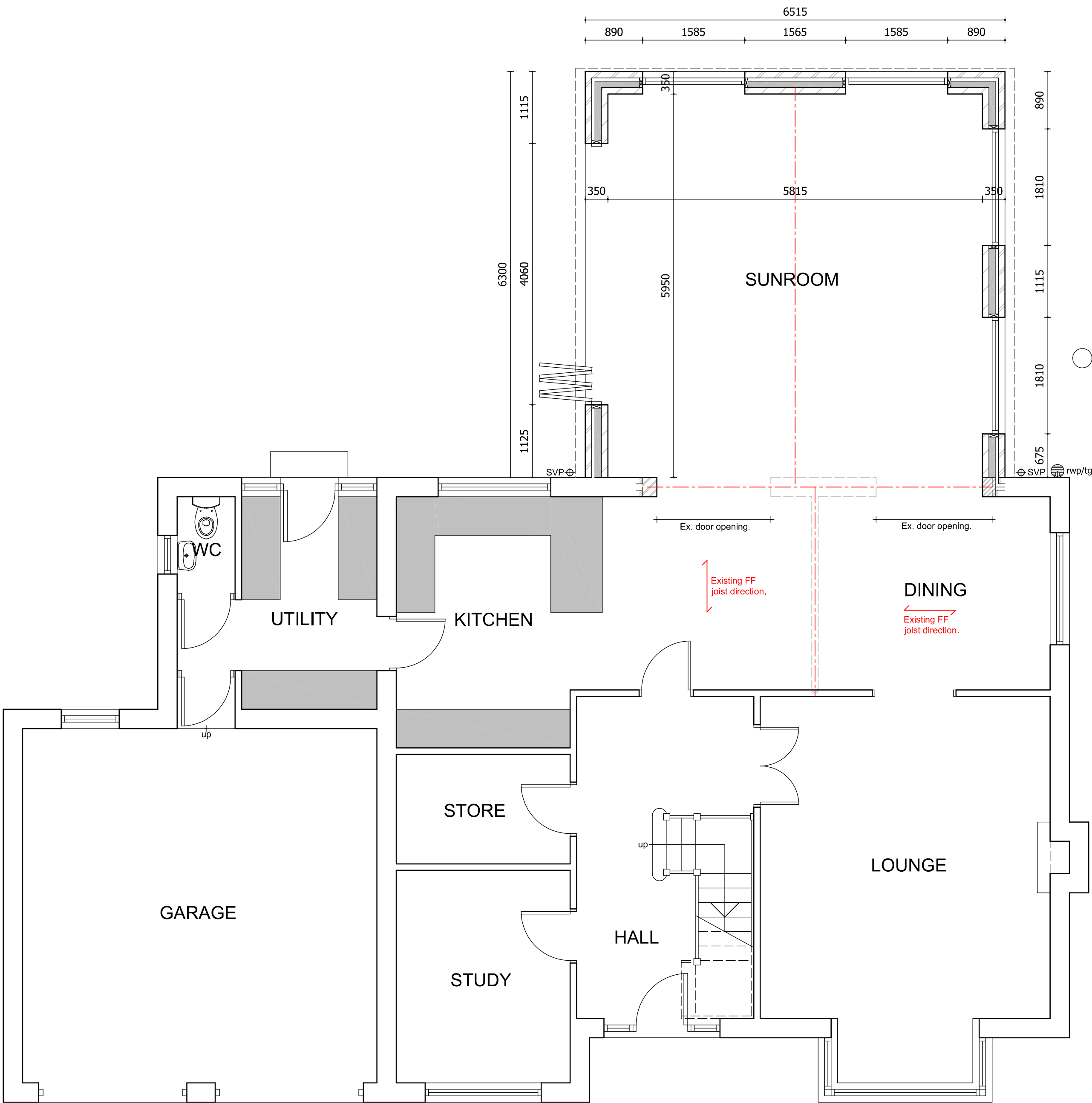
GF PLAN
