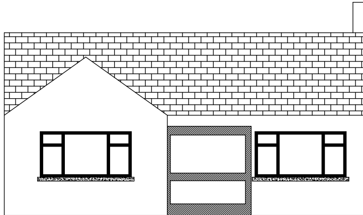
EXISTING FRONT ELEVATION SCALE 1:100
