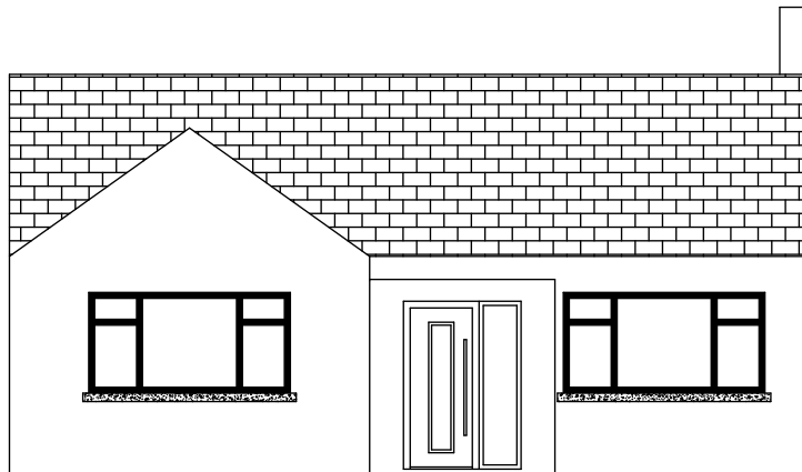
PROPOSED FRONT ELEVATION SCALE 1:100
