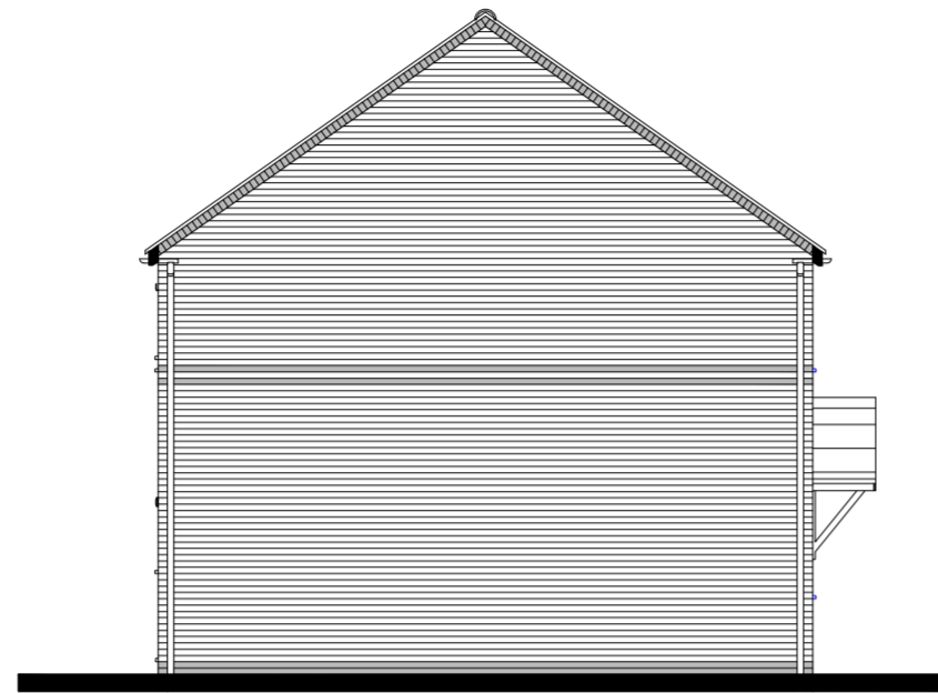
201 SIDE ELEVATION
