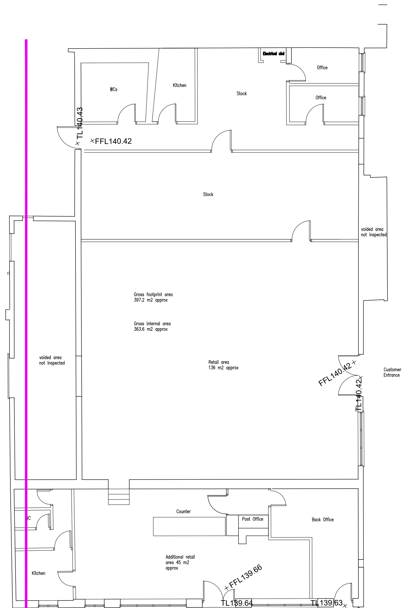
Existing Plan
