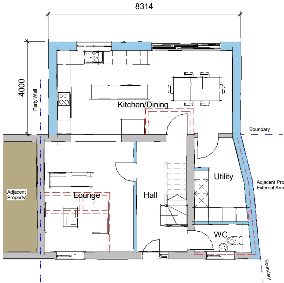
Ground 1 : 100
