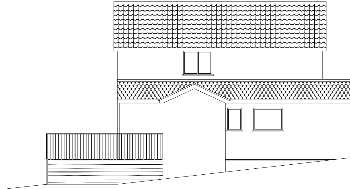
West elevation
