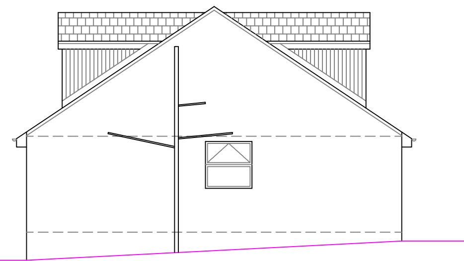
Side Elevation
