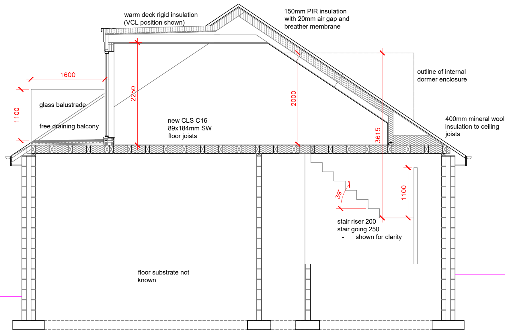
Section
