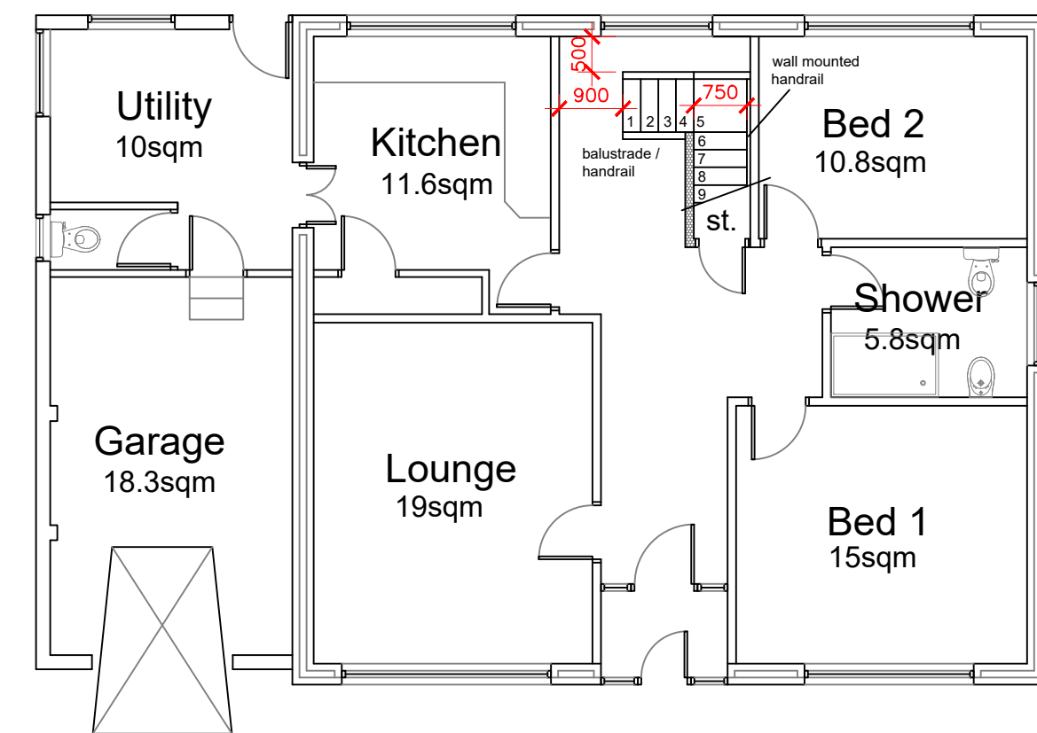
Floor Plan
