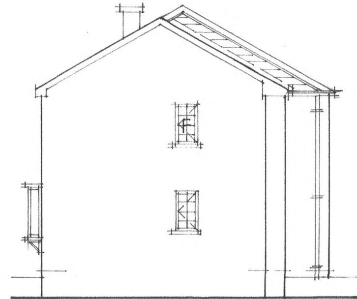
SIDE 1:100 ELEVATIONS
