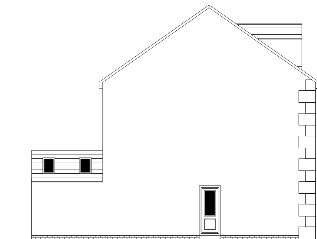
SOUTH ELEVATION PLOT 3
