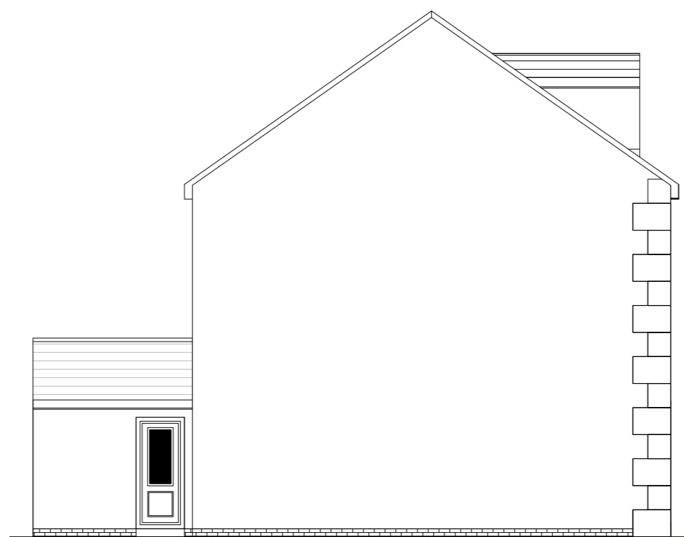
SOUTH ELEVATION PLOT 2
