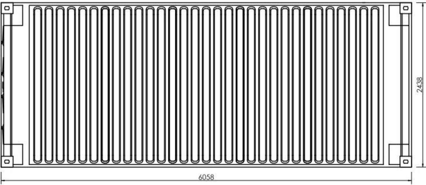
20ft Shipping Container - Roof Plan
