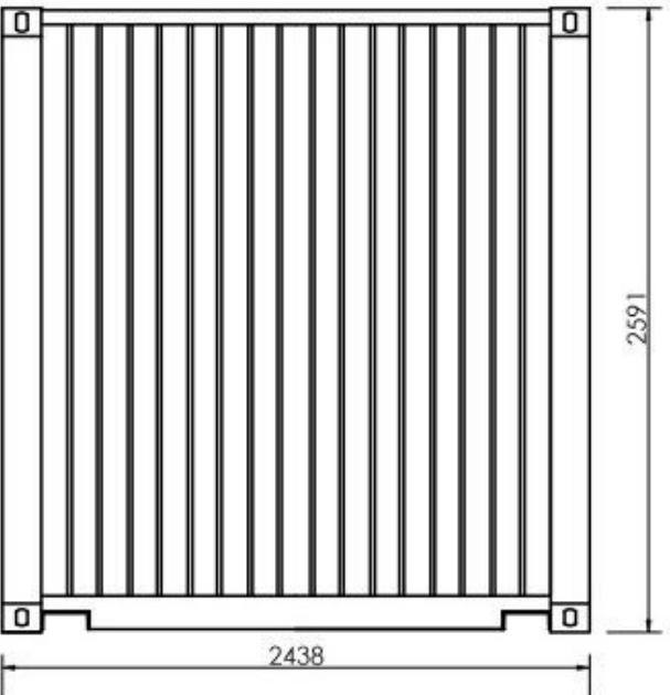
20ft Shipping Container - Front Elevation
