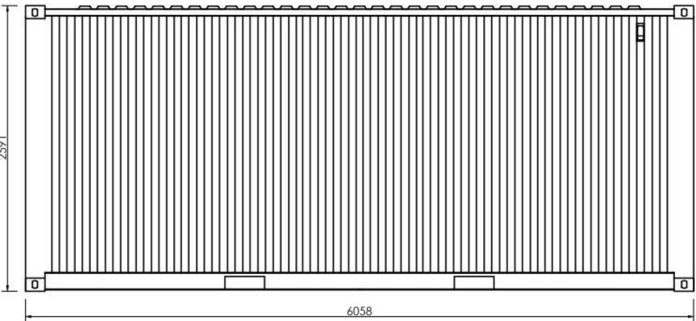
20ft Shipping Container - Side Elevation
