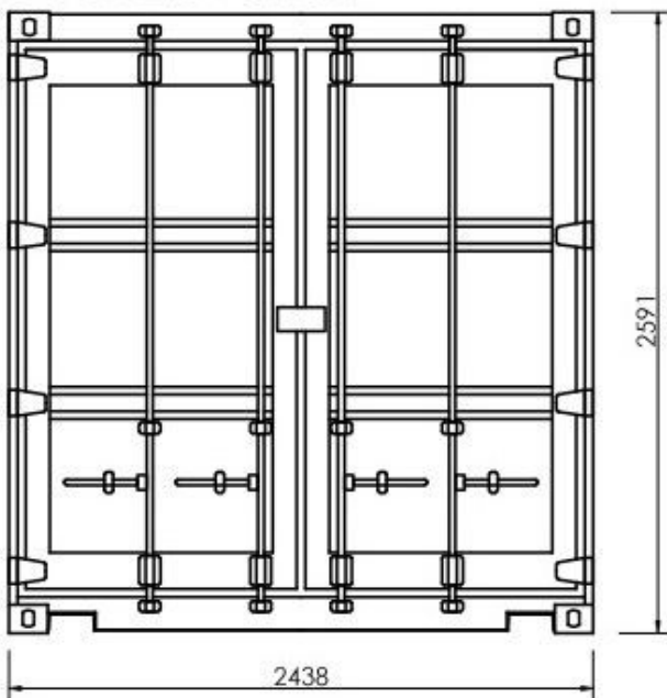
20ft Shipping Container - Door Elevation
