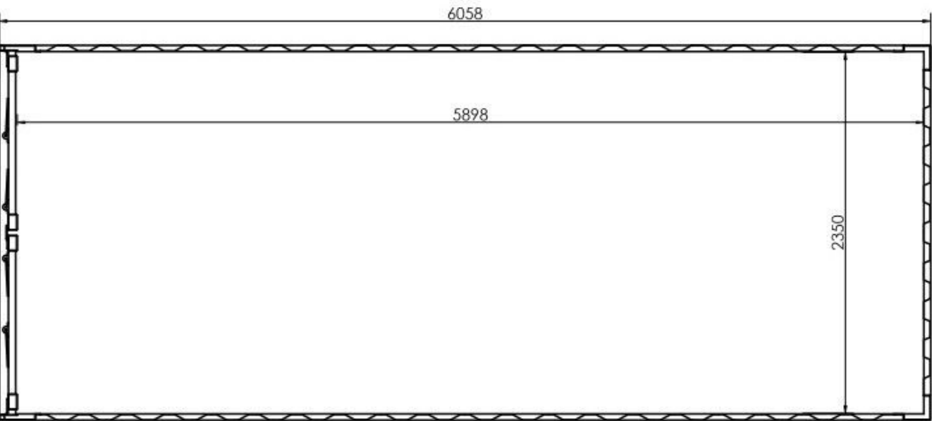
20ft Shipping Container - Plan
