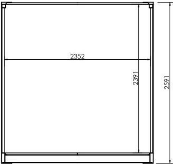
20ft Shipping Container - Section
