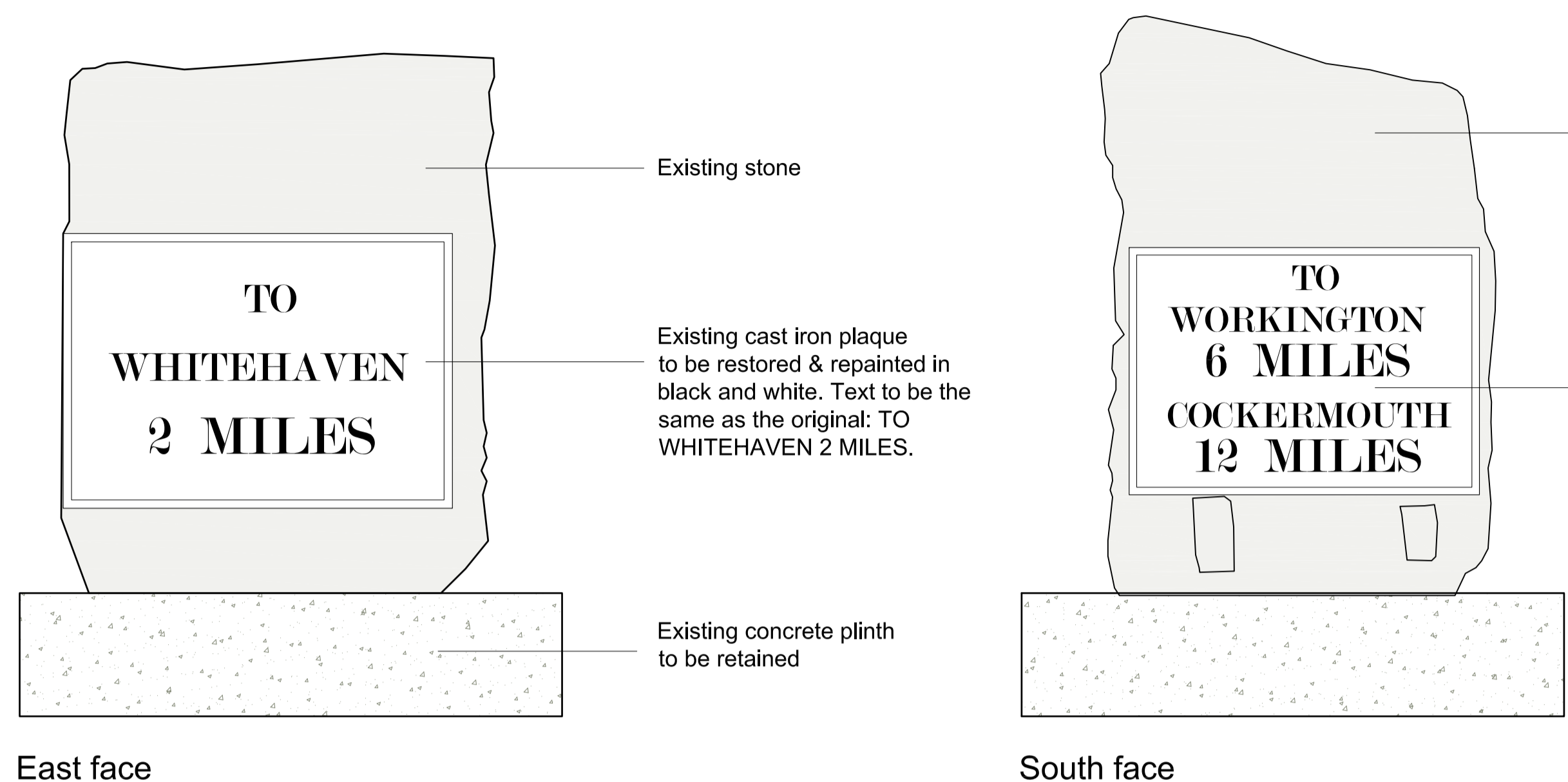
Proposed Elevations. NTS
