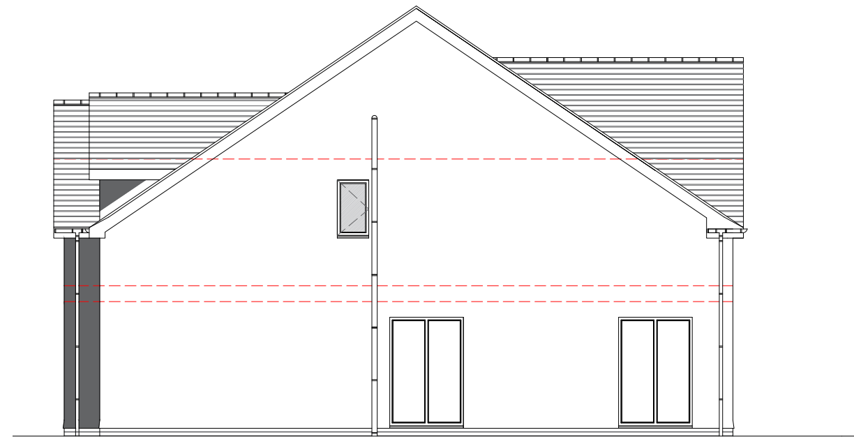
North Elevation
