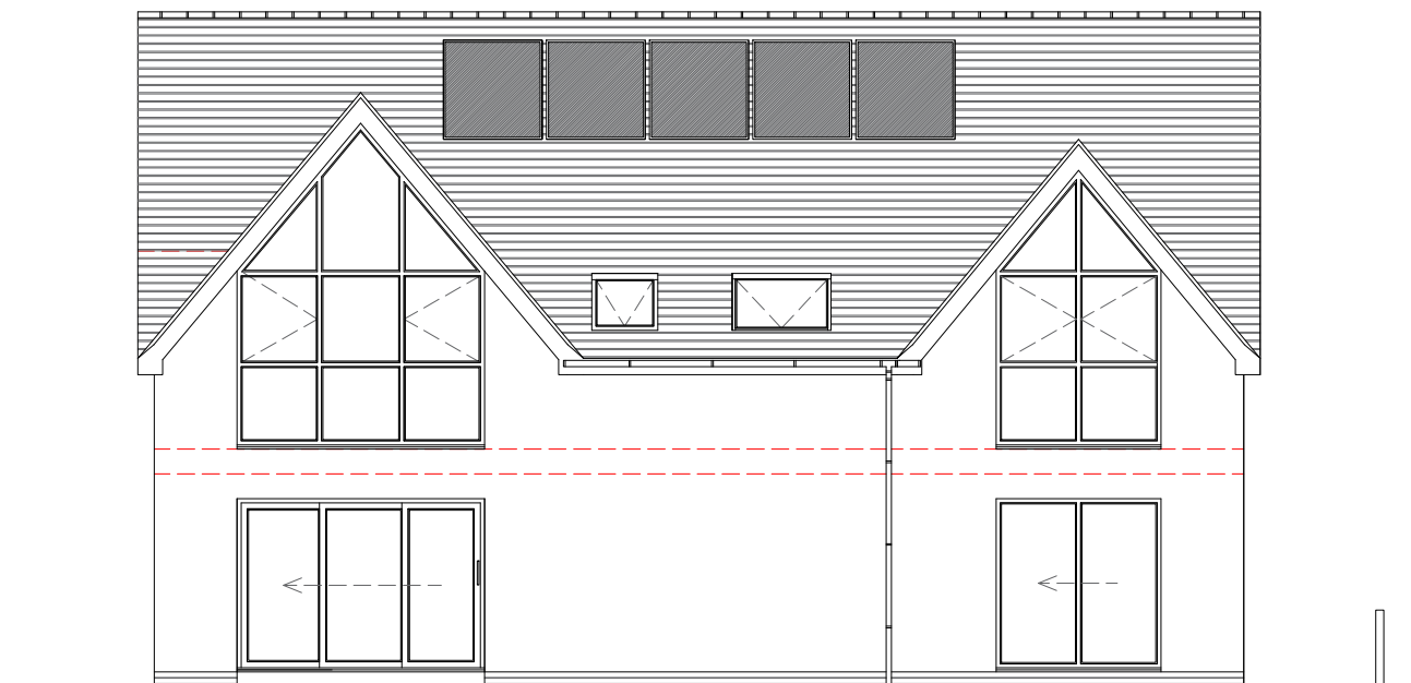
West Elevation
