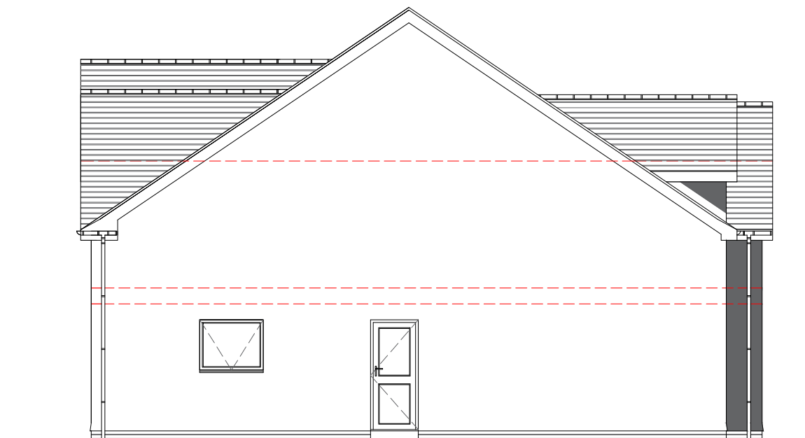
South Elevation
