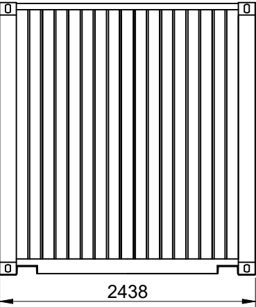
20ft Shipping Container - Door Elevation
