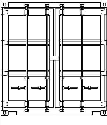
20ft Shipping Container - Door Elevation
