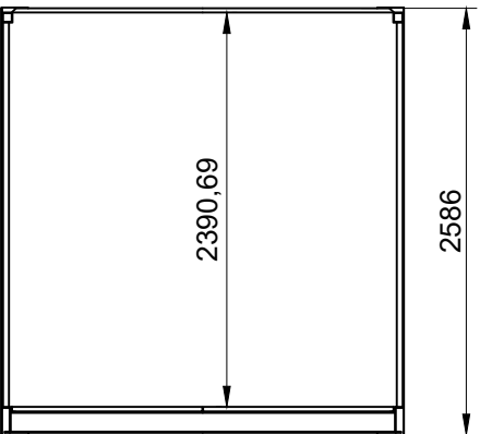
20ft Shipping Container - Section
