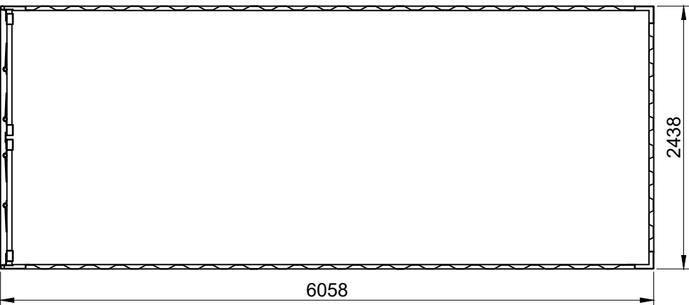
20ft Shipping Container - Roof Plan
