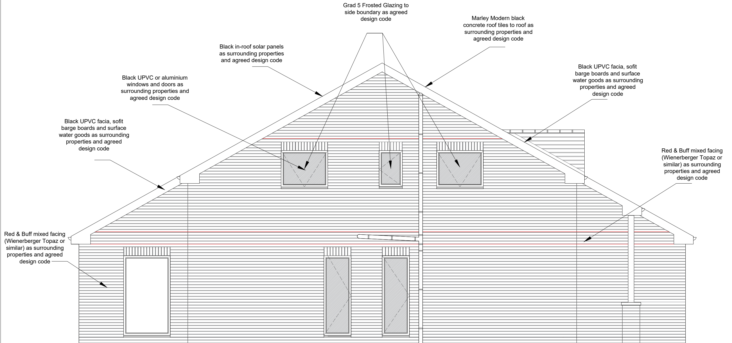
South Elevation
