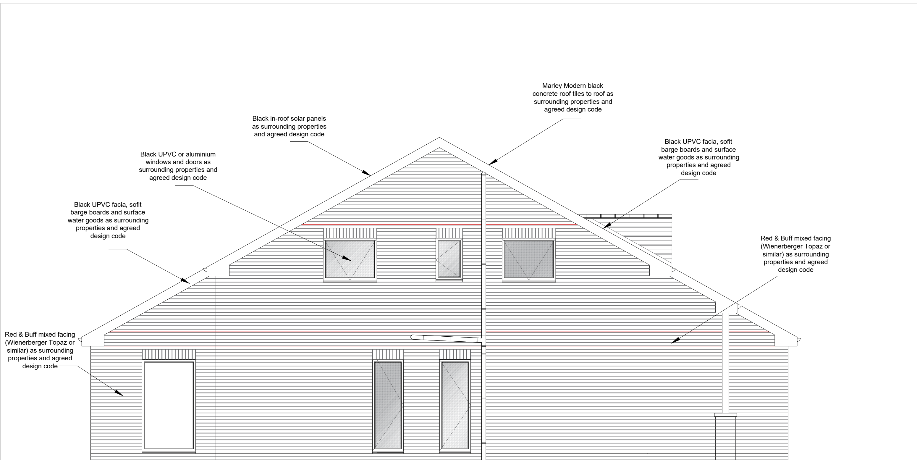
South Elevation
