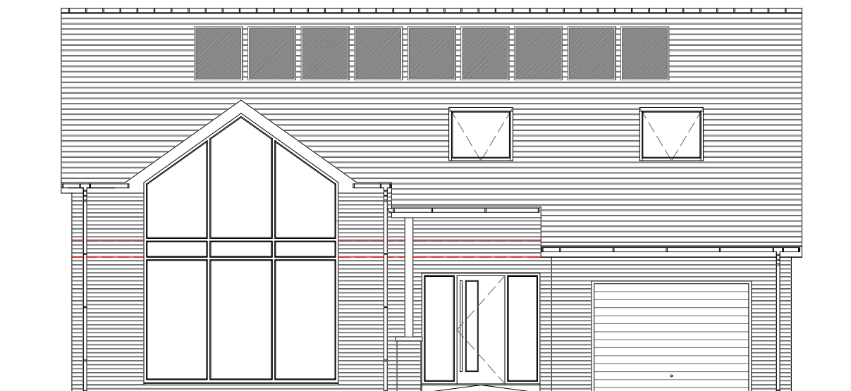
East Elevation
