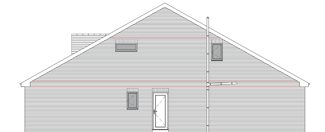
North Elevation
