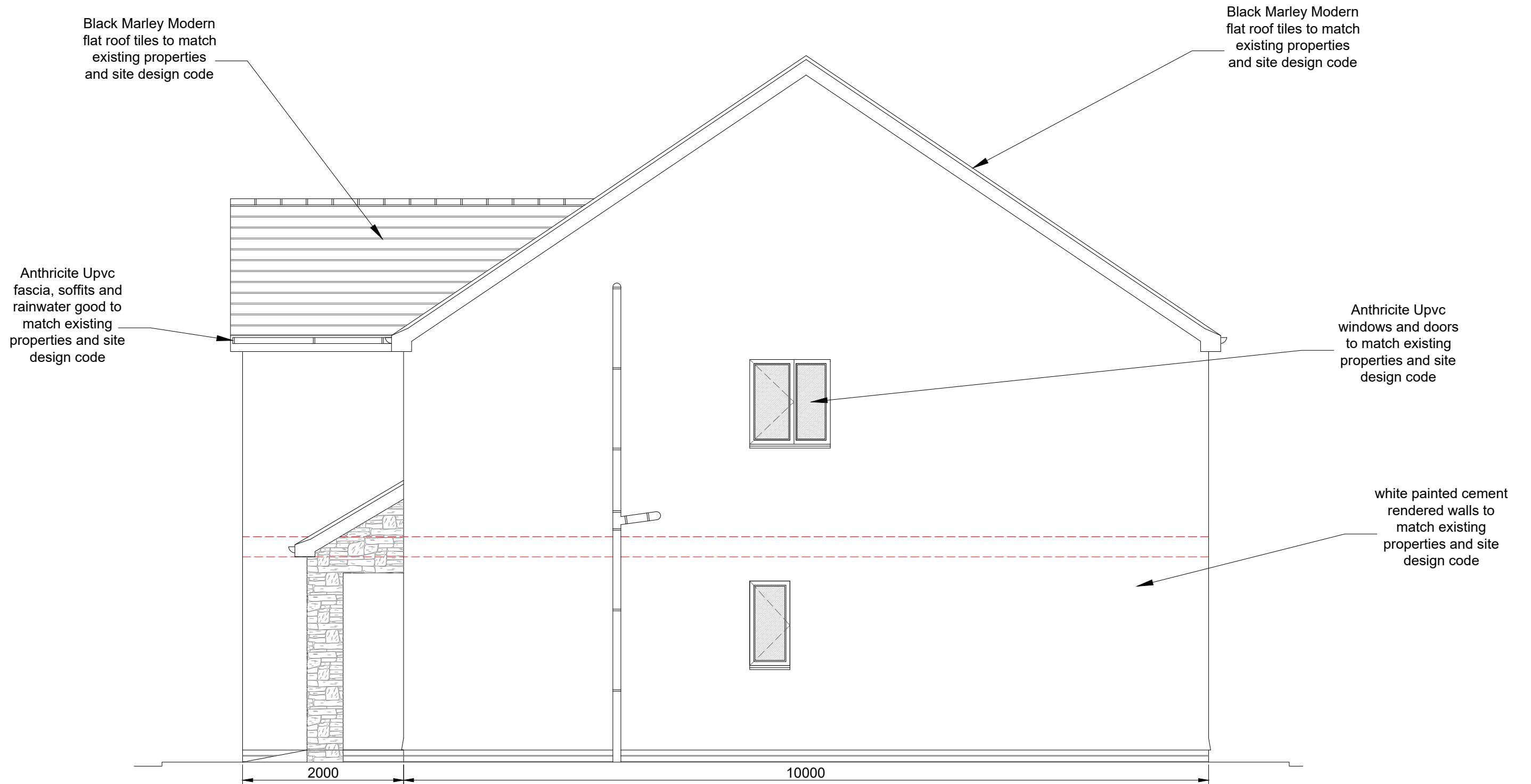
East Elevation
