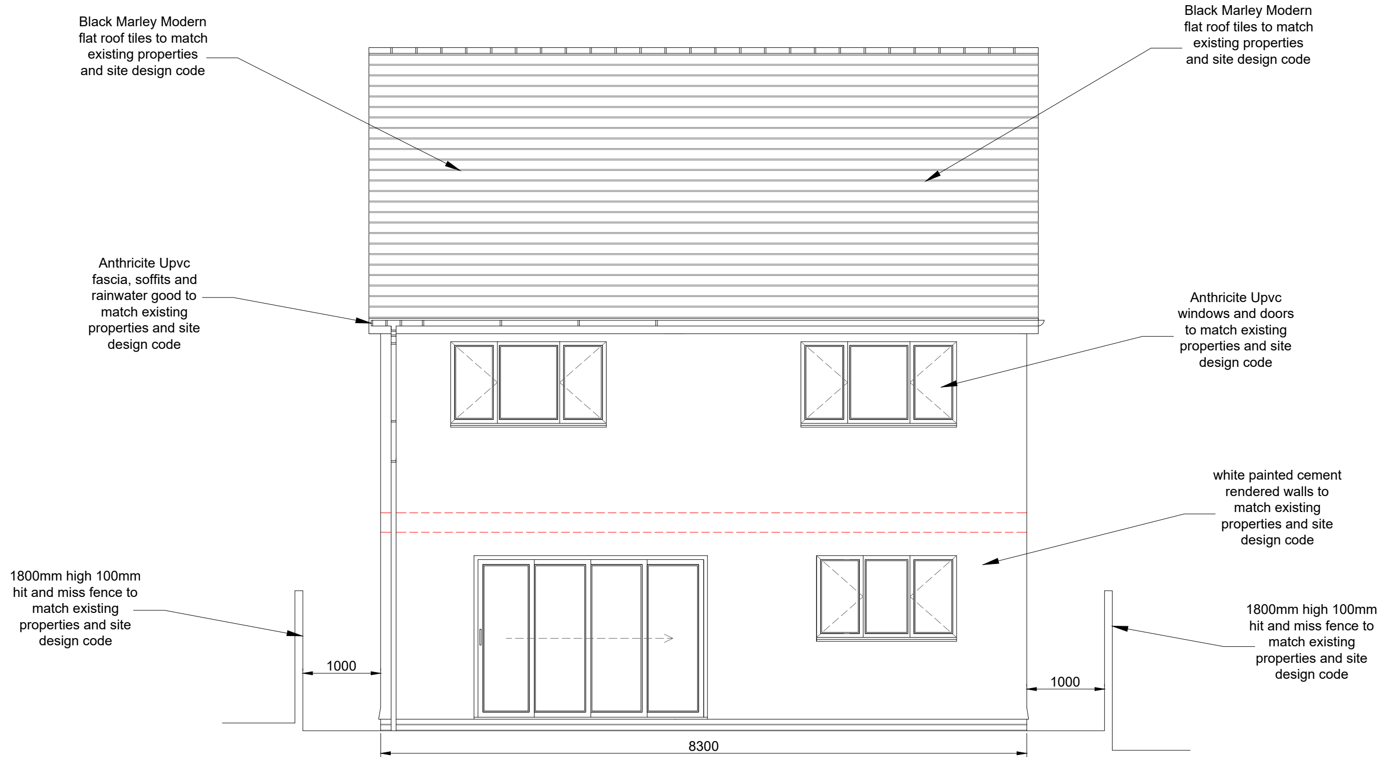
North Elevation
