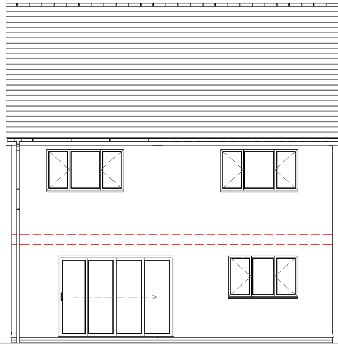
North Elevation
