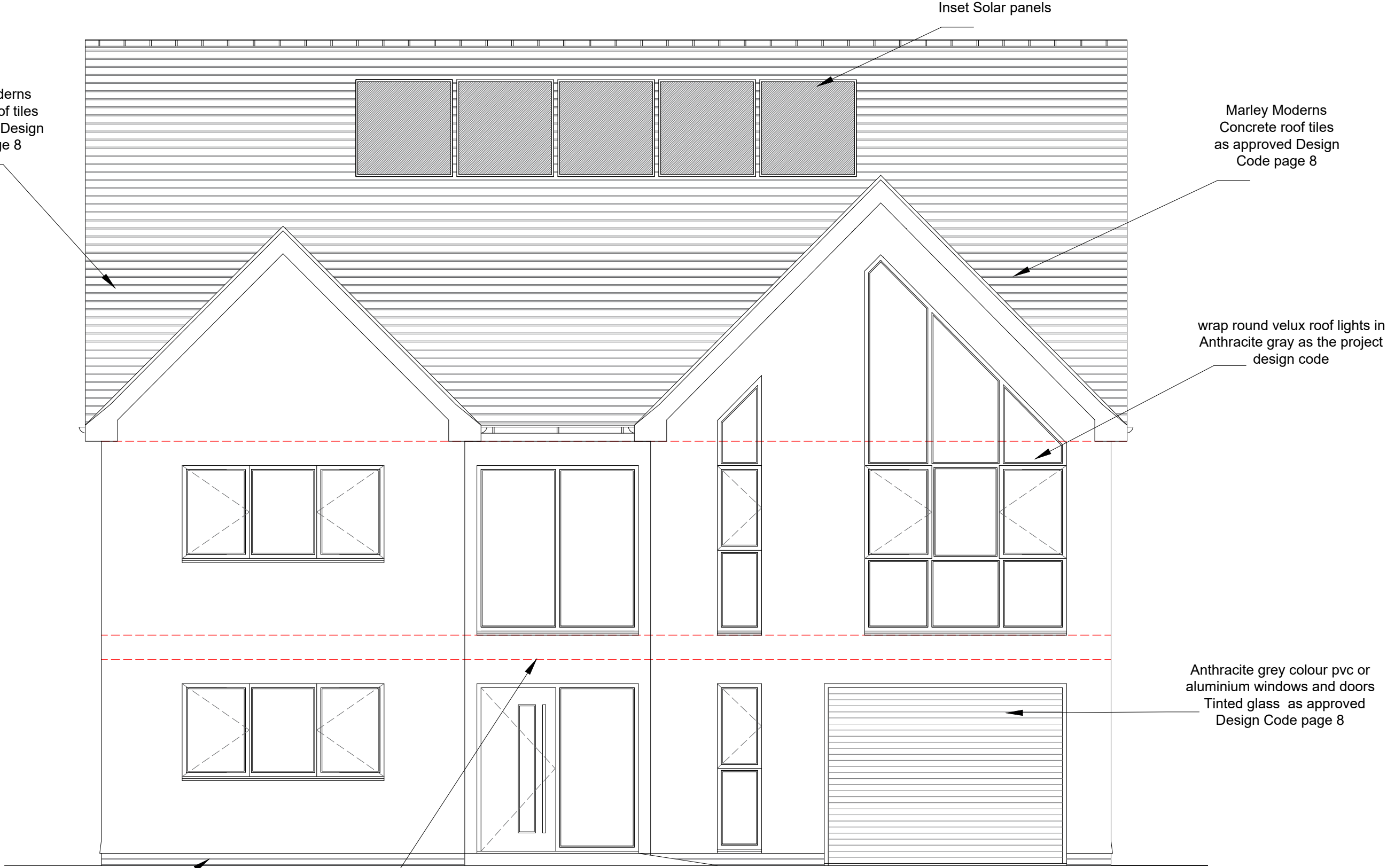
West Elevation
