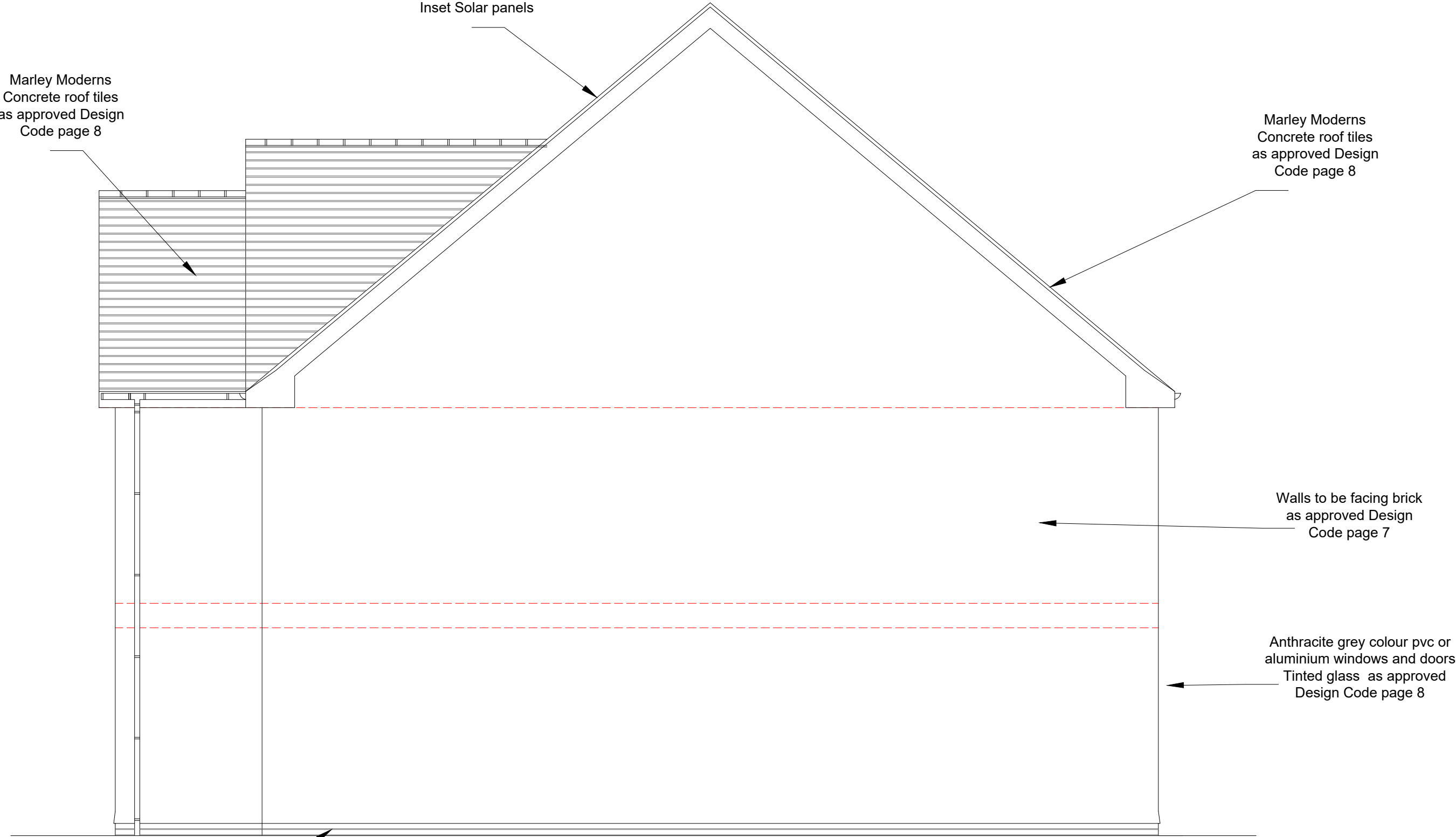
South Elevation
