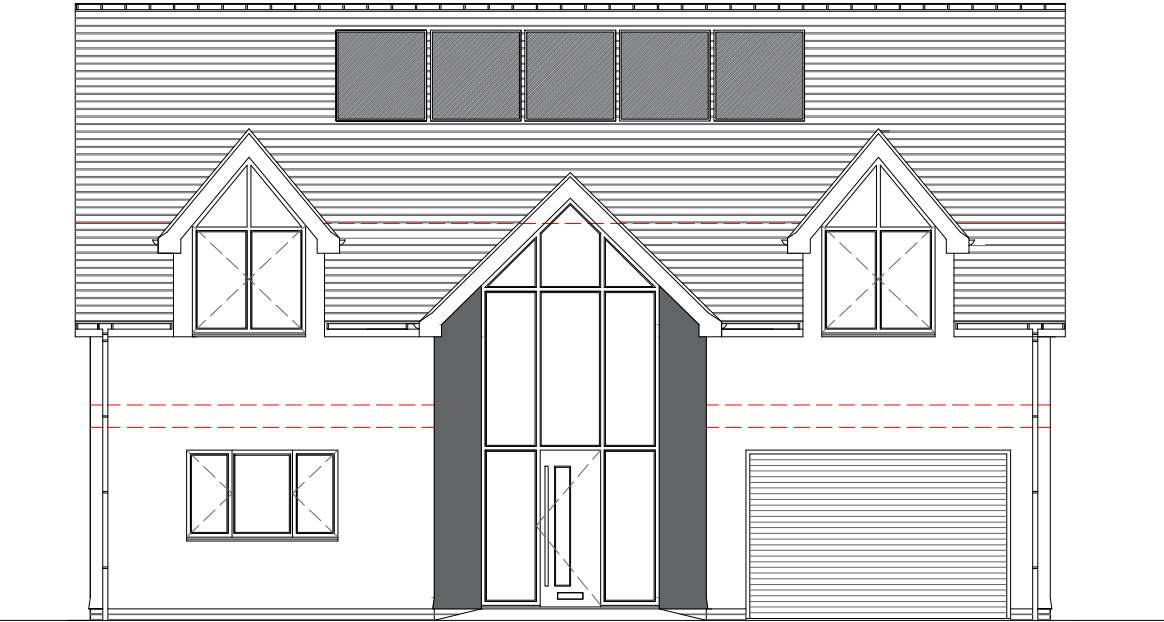
East Elevation
