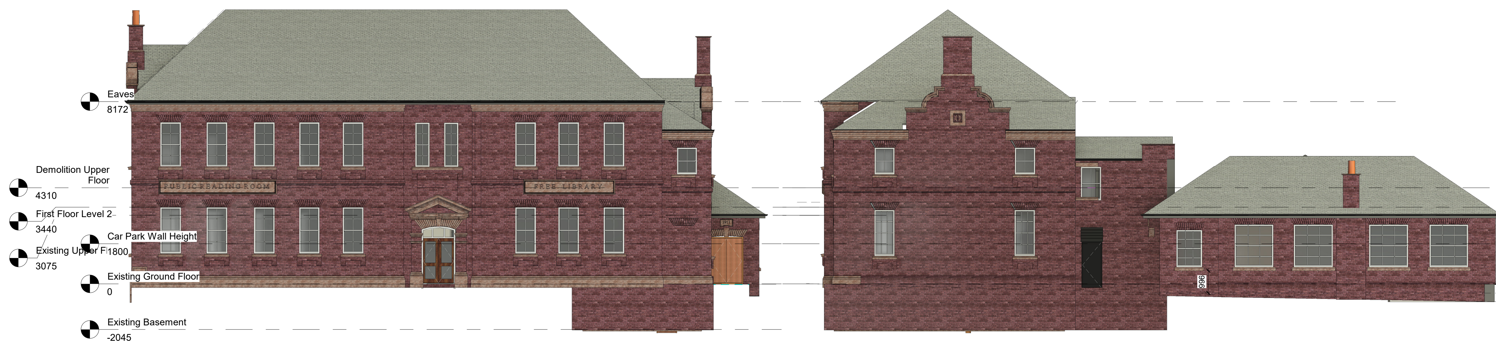
2 Proposed Elevation 2
