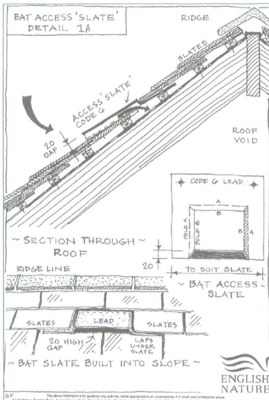
Slate access provision to western slope of barn A
