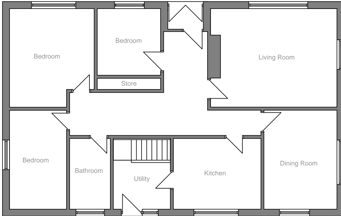
FIRST FLOOR (SPLIT LEVEL)
