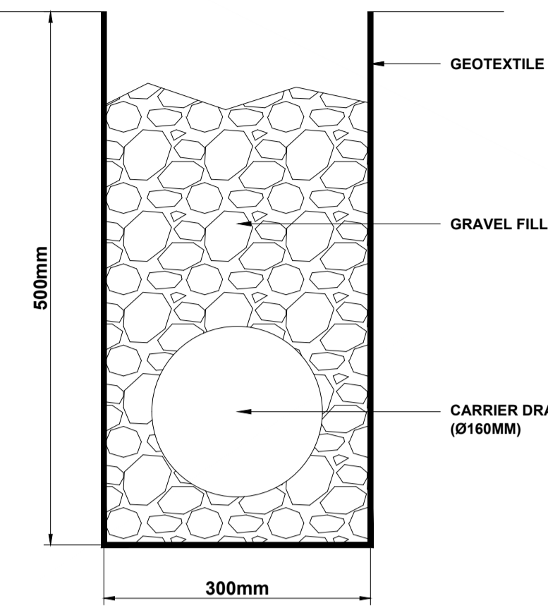
CARRIER DRAIN SECTION SCALE 1:5
