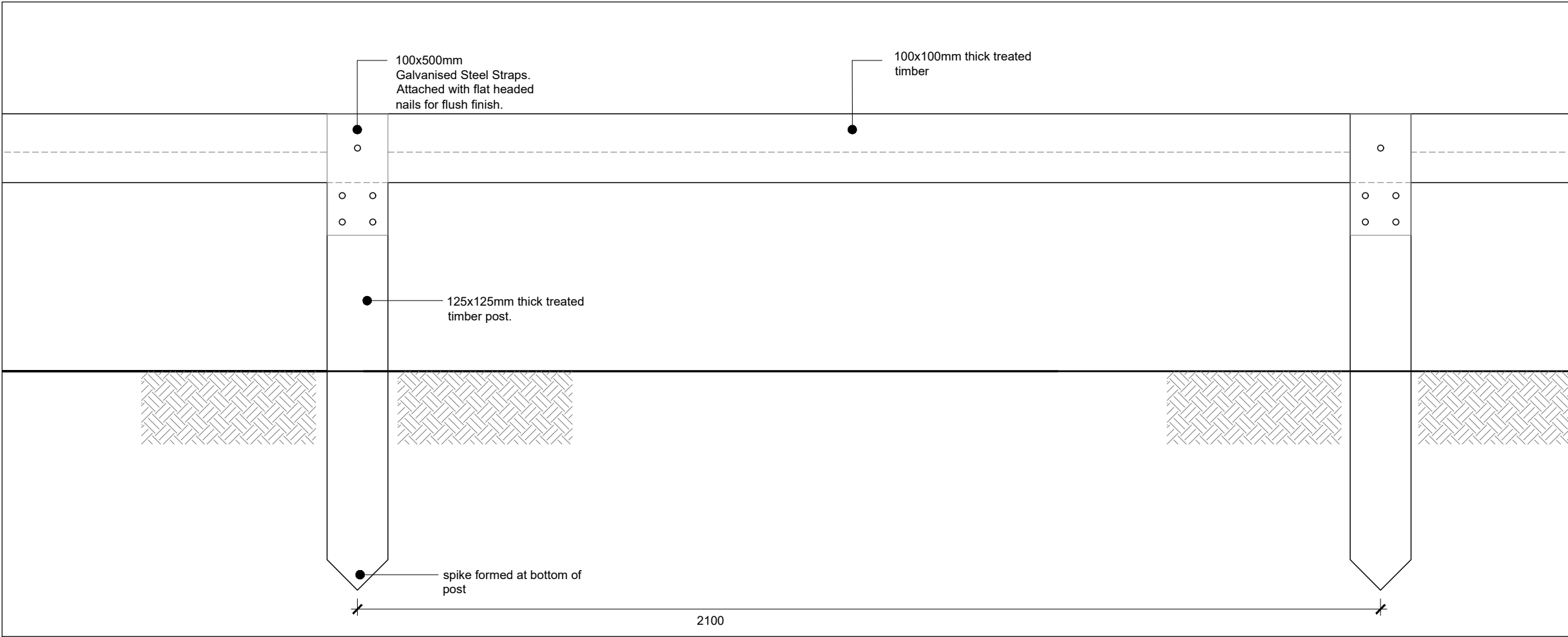
TYPICAL ELEVATION 1:10
