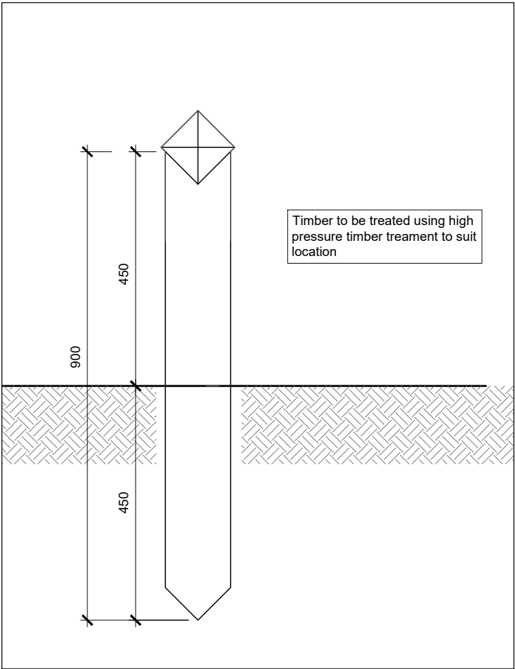
TYPICAL SECTION 1:10
