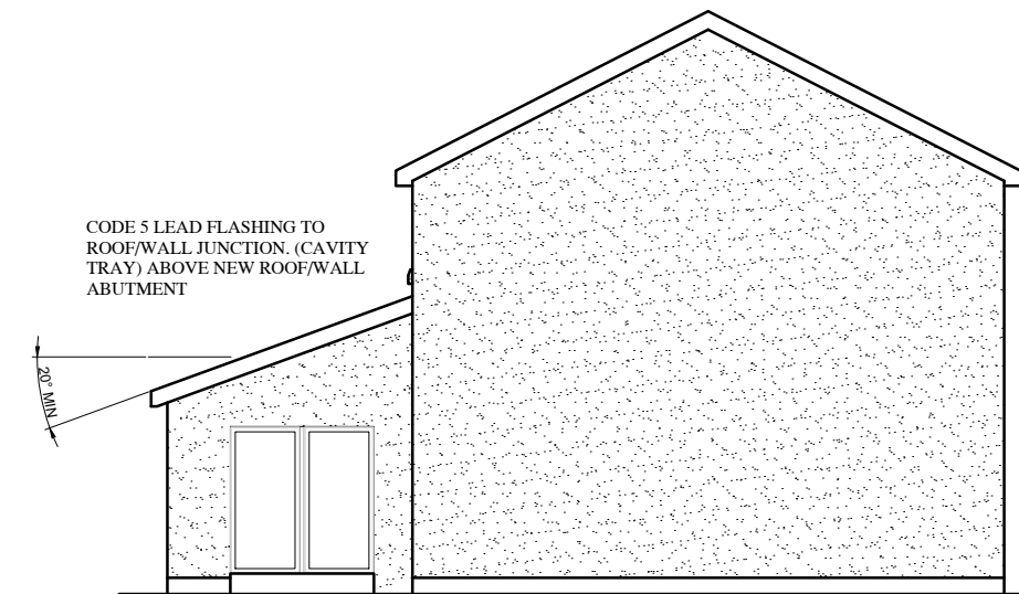
PROPOSED GABLE ELEVATION
