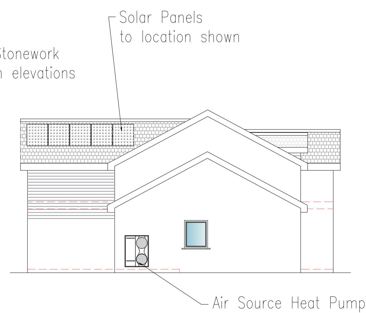
Side Elevation
