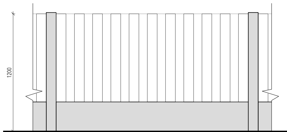
1200 High Hit & Miss Fence with Gravel Board (1:20)
