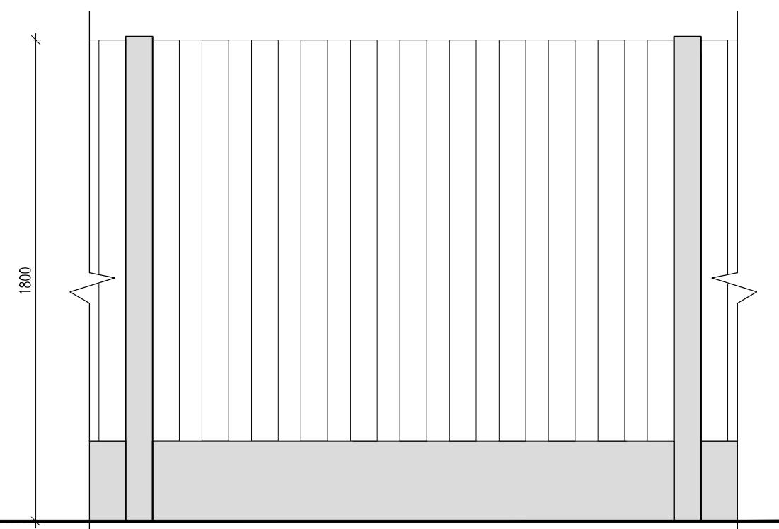
1800 High Hit & Miss Fence with Gravel Board (1:20)
