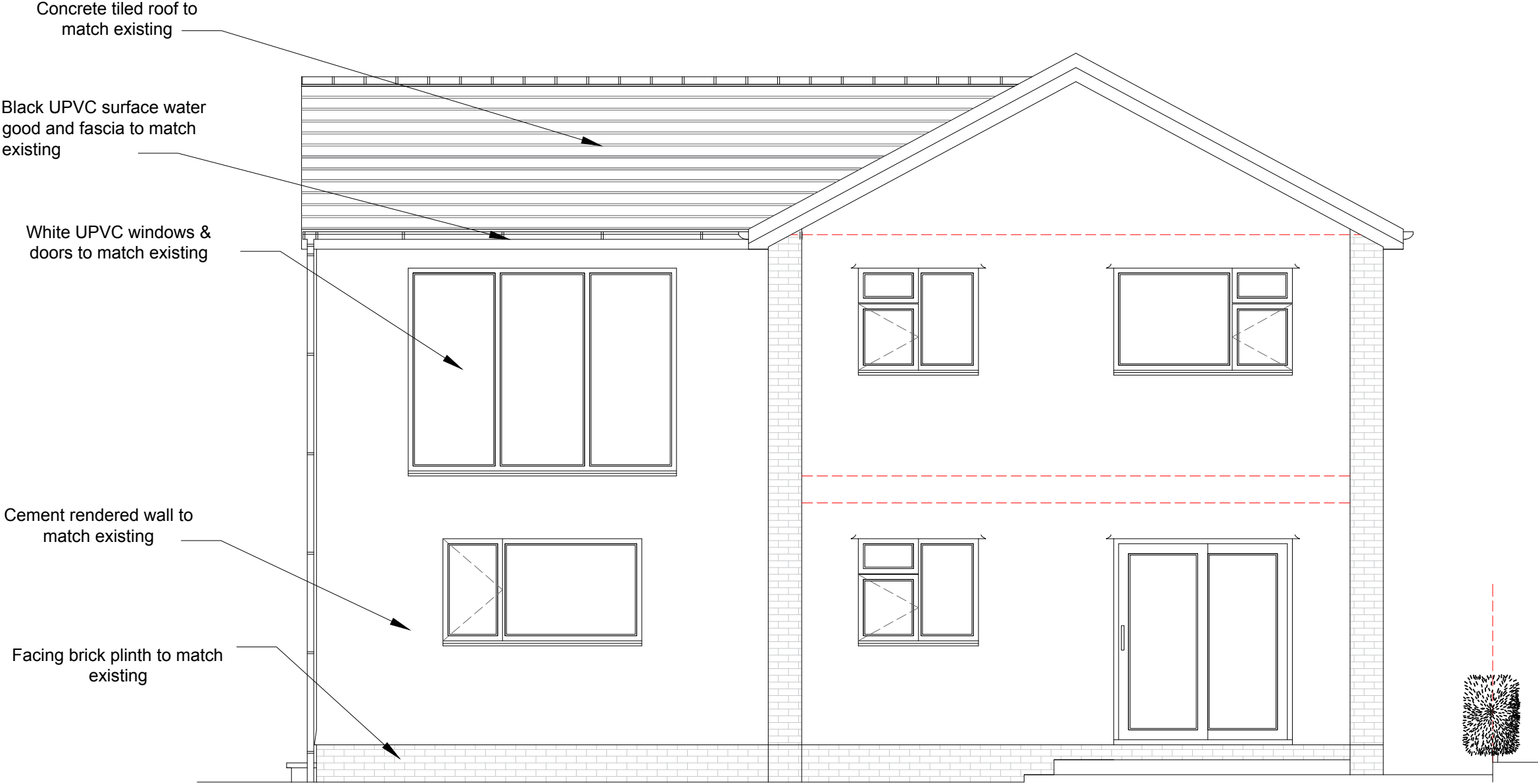
North Elevation
