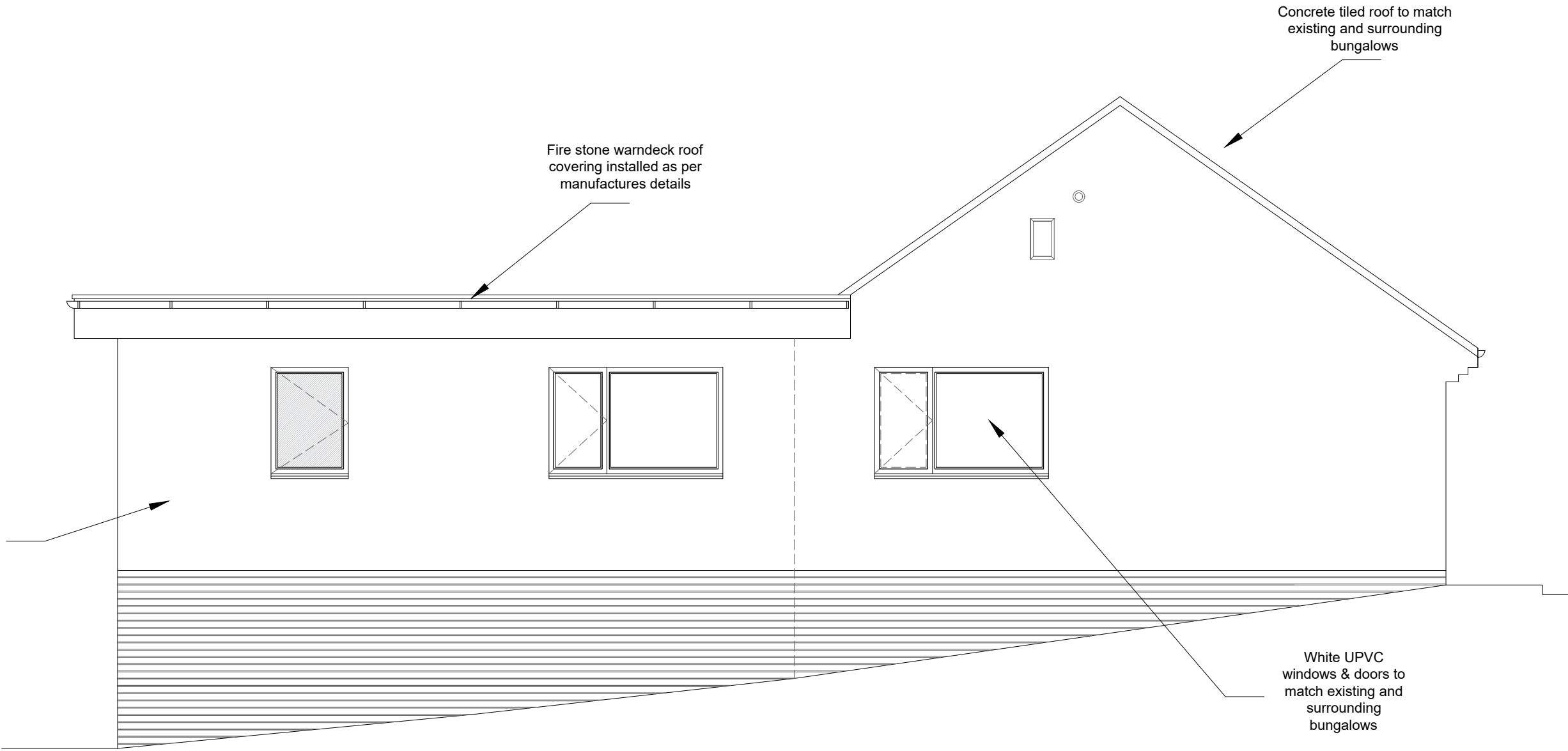
North Elevation
