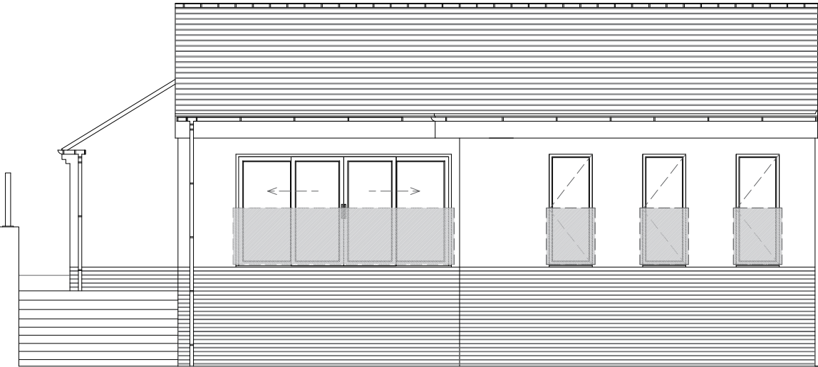
East Elevation
