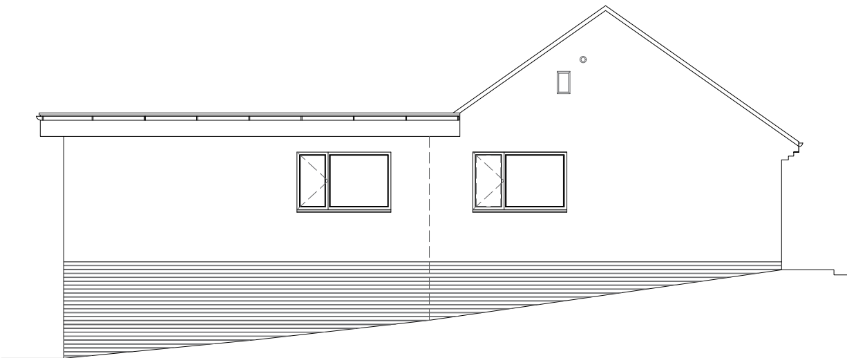
East Elevation
