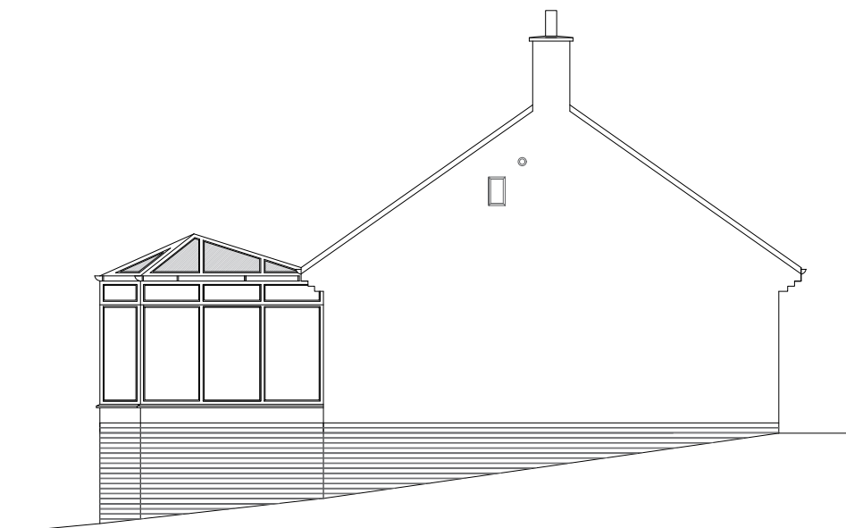
North Elevation
