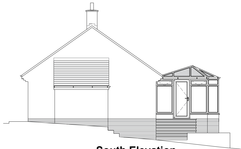
South Elevation
