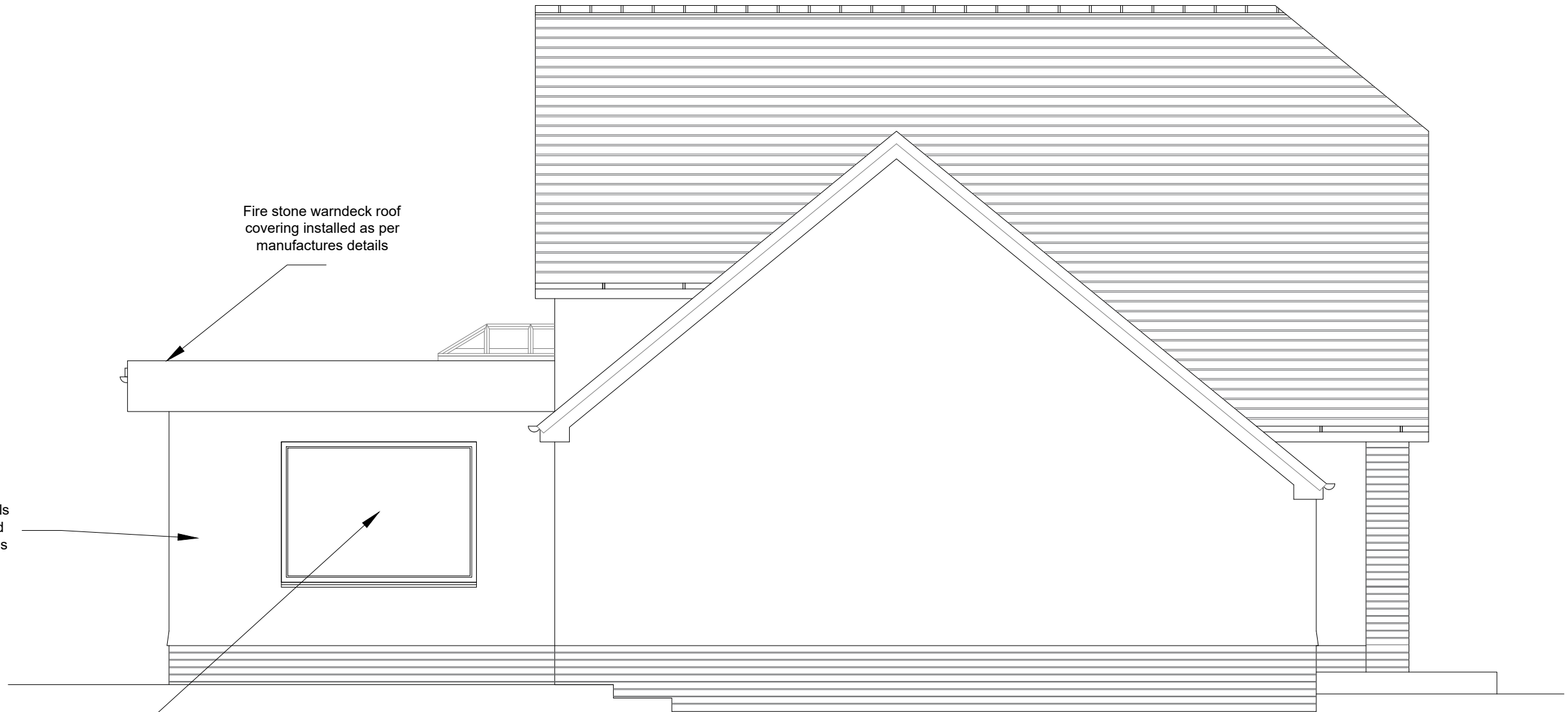
North Elevation
