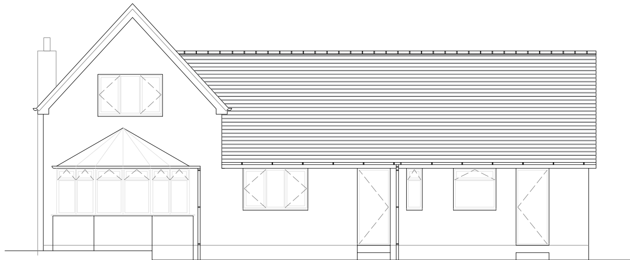
East Elevation
