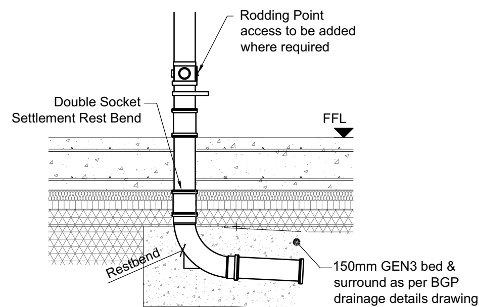
Typical Detail through Internal Pop-Up (PU) NTS
