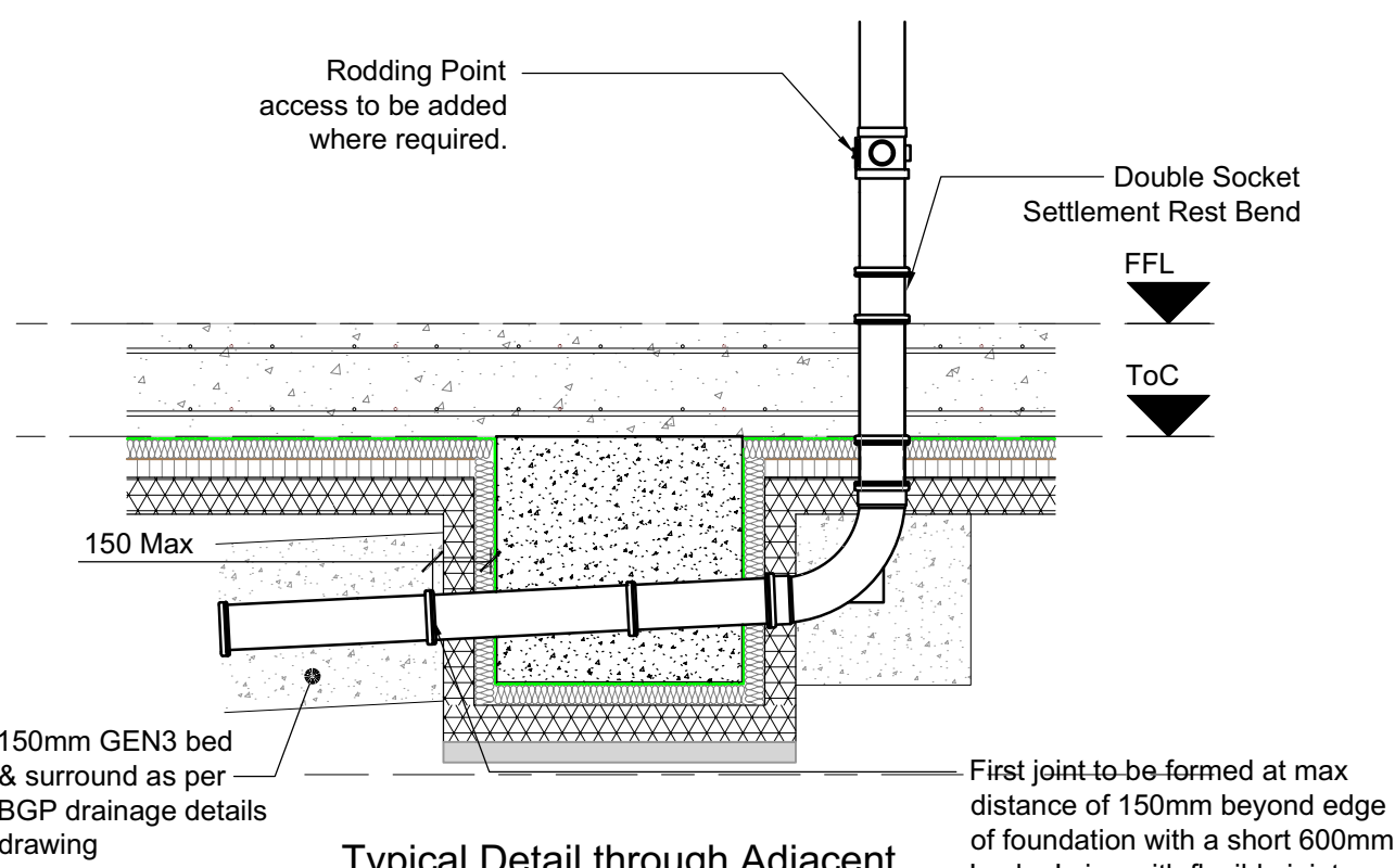
Typical Detail through Adjacent Internal Ground Beam Pop-Up (PU) NTS
