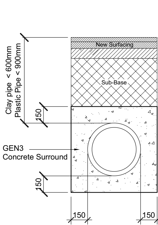
Concrete Surround Detail (Hardstanding areas & beneath building slab)
