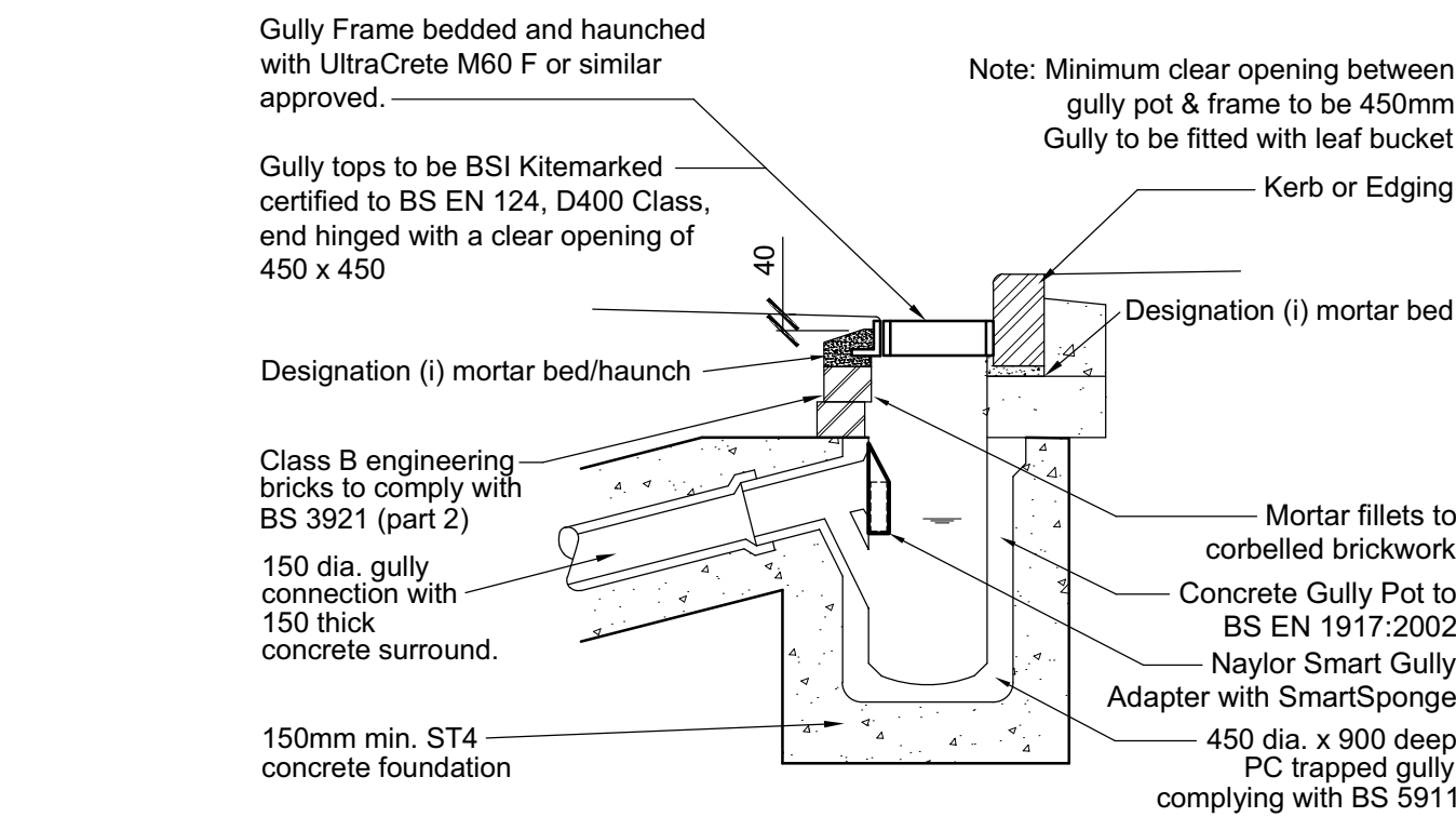
Naylor Concrete Smart Gully Detail (G) NTS
