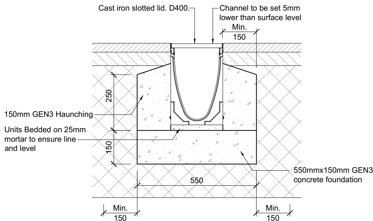
Typical ACO MultiDrain MD with M200D 0.0 Channel (or similar approved) Scale 1:10
