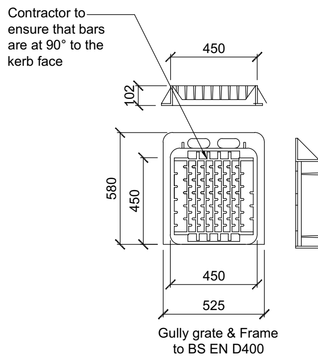
Road Gully Grating (For Highways Adoption) NTS
