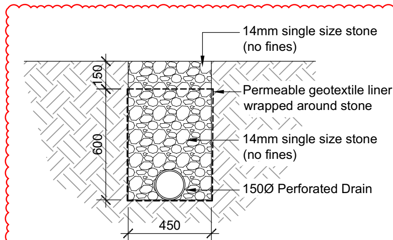
Typical Section Through Filter Drain
