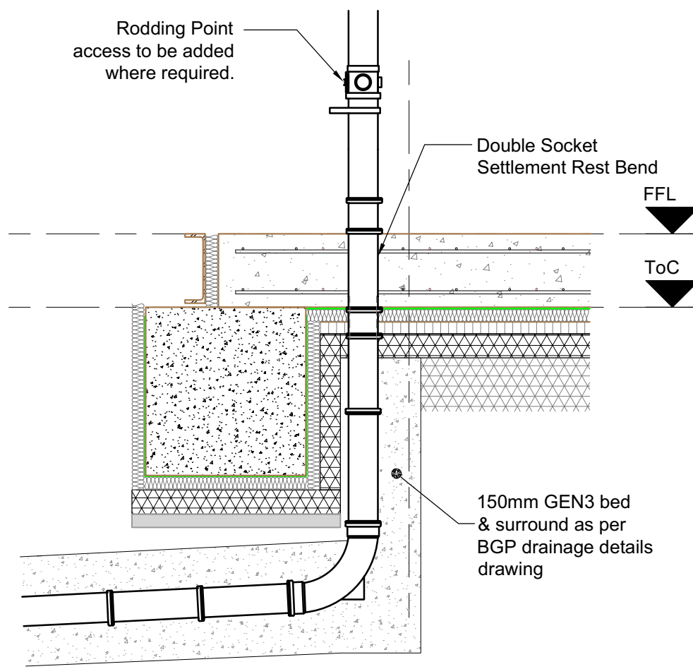
Typical Detail showing Pop Up Beneath Perimeter Ground Beam Foundation NTS
