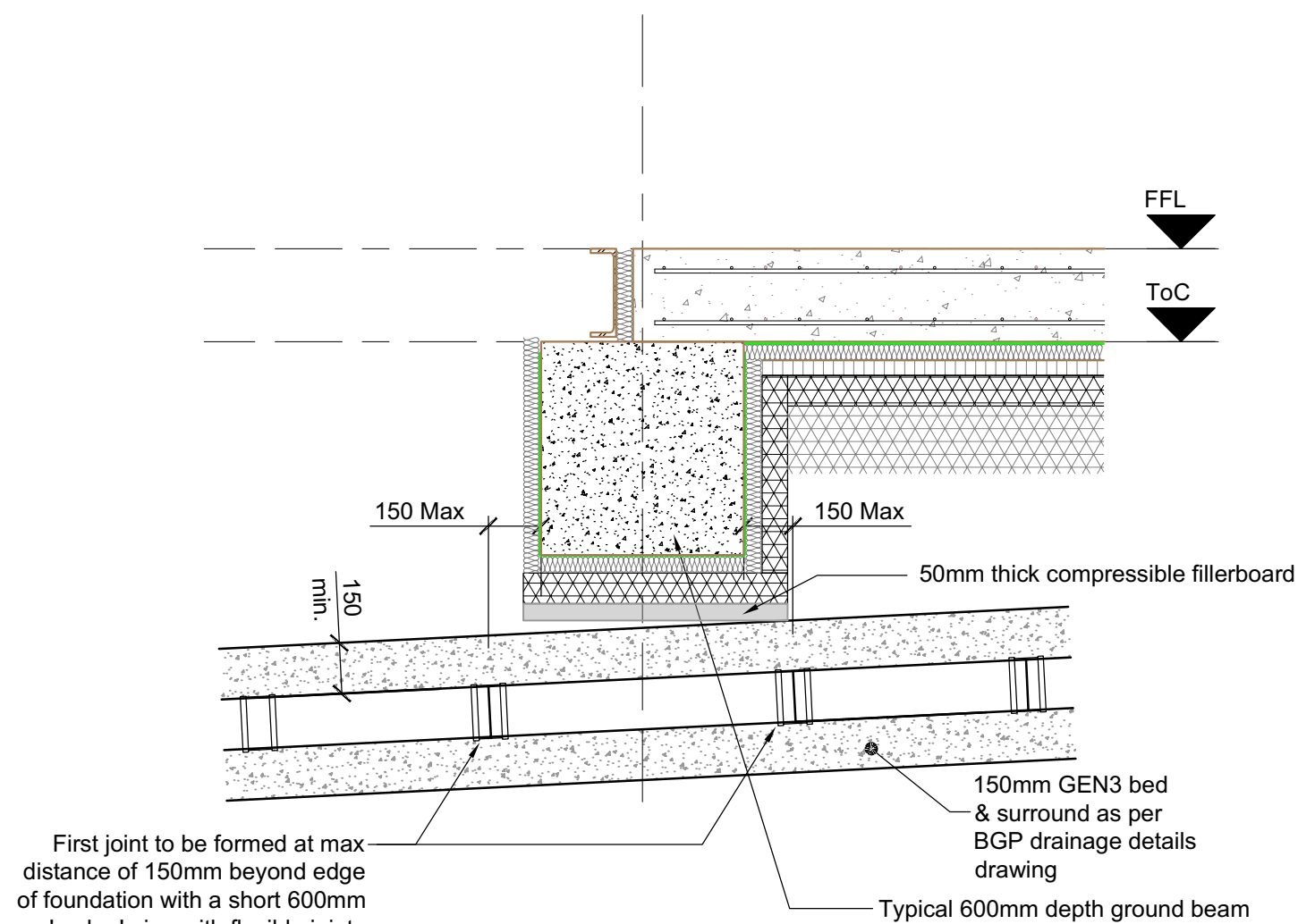
Typical Detail showing Pipe beneath Ground Beam Foundation NTS
