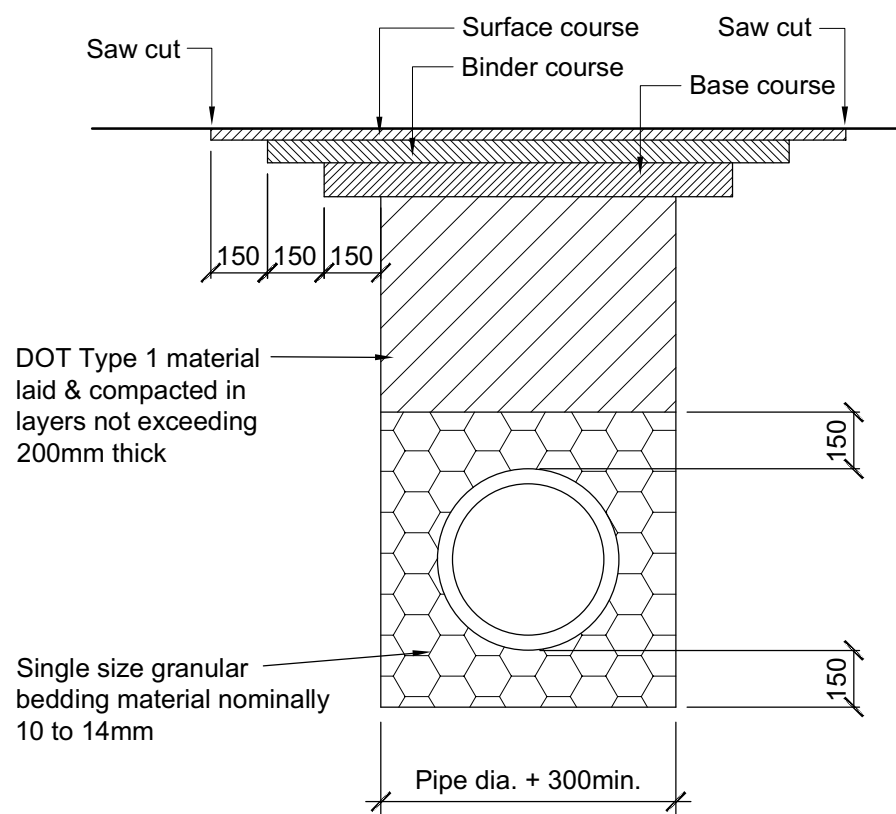
Carriageway Reinstatement Detail Scale 1:20
