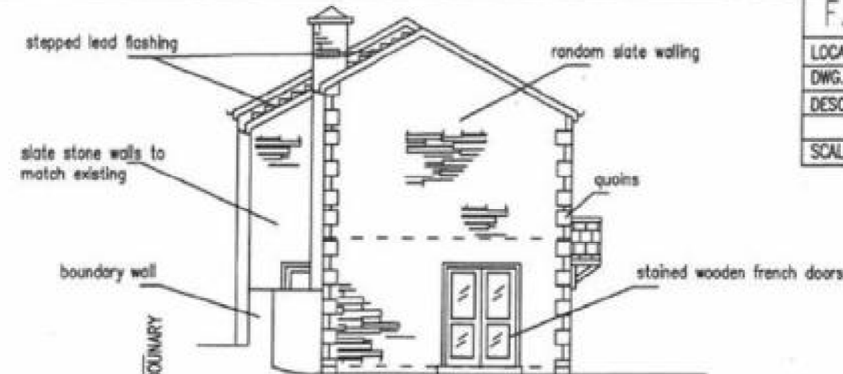
SIDE ELEVATION
