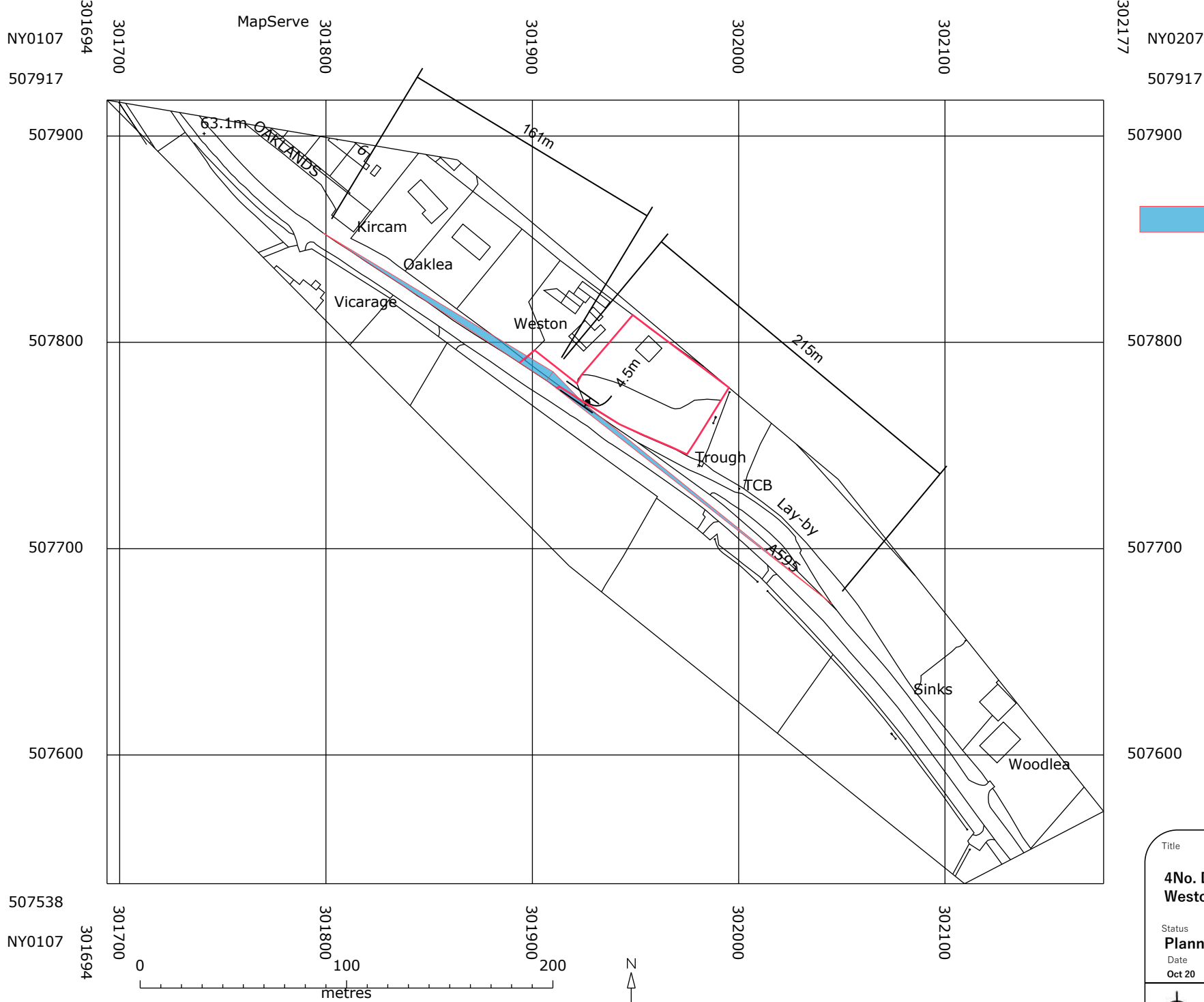
Location Plan 1:2500
