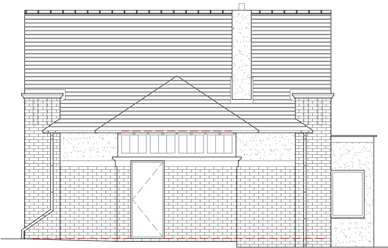
West Elevation
