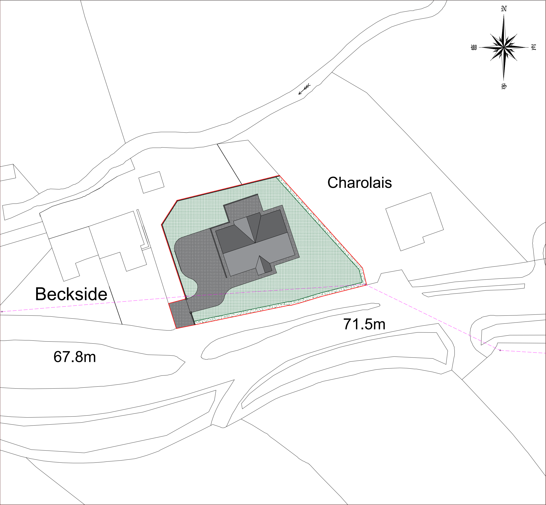
Block Plan 1/500
