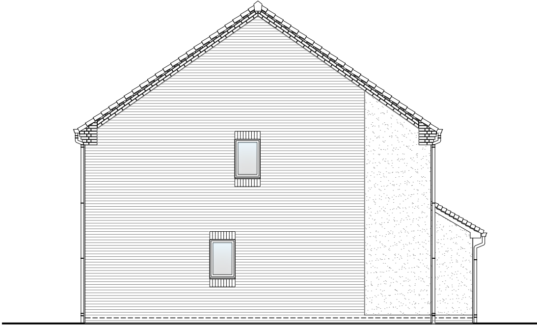
Left Elevation
