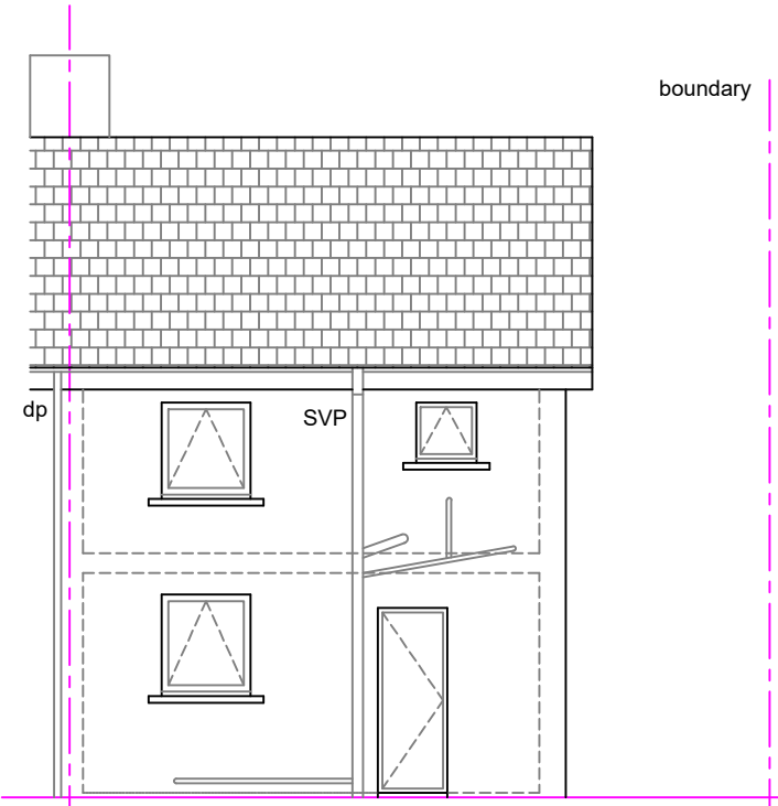
Rear Elevation
