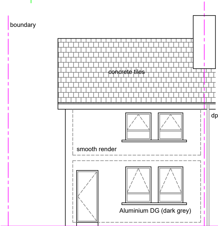
Front Elevation
