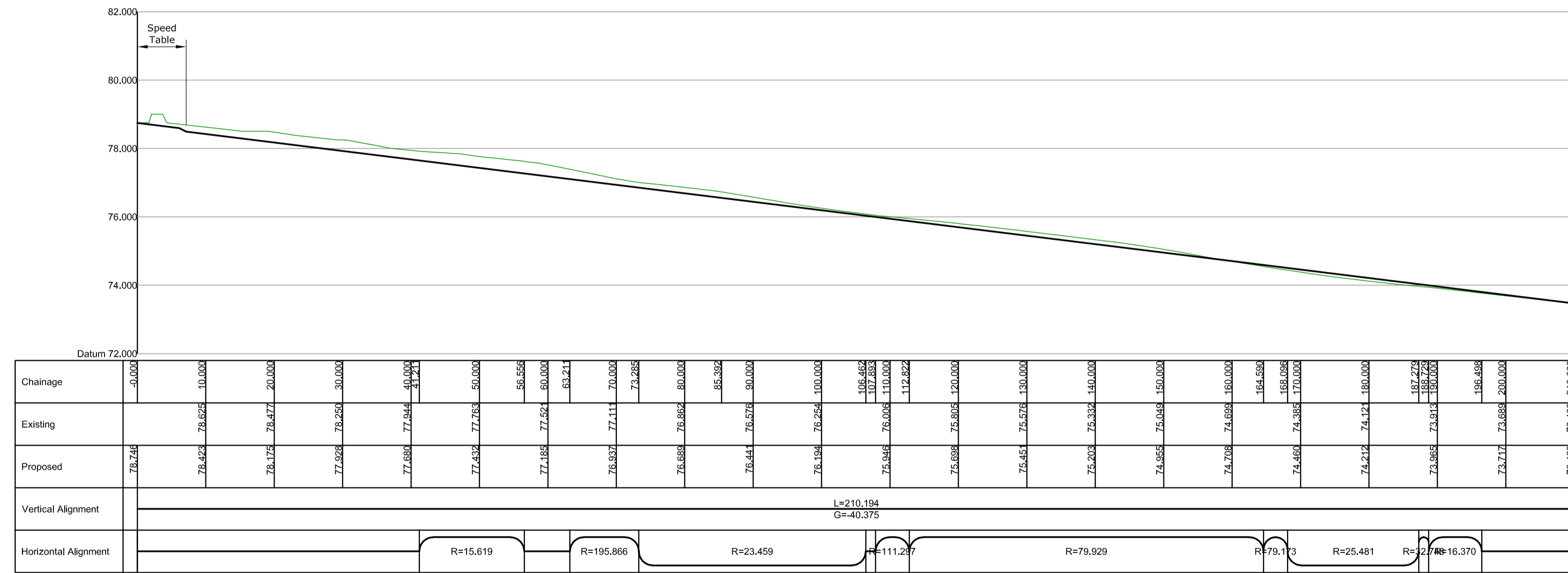
Longitudinal Section Along Main Road Scale 1:500 Horizontal 1:100 Vertical
