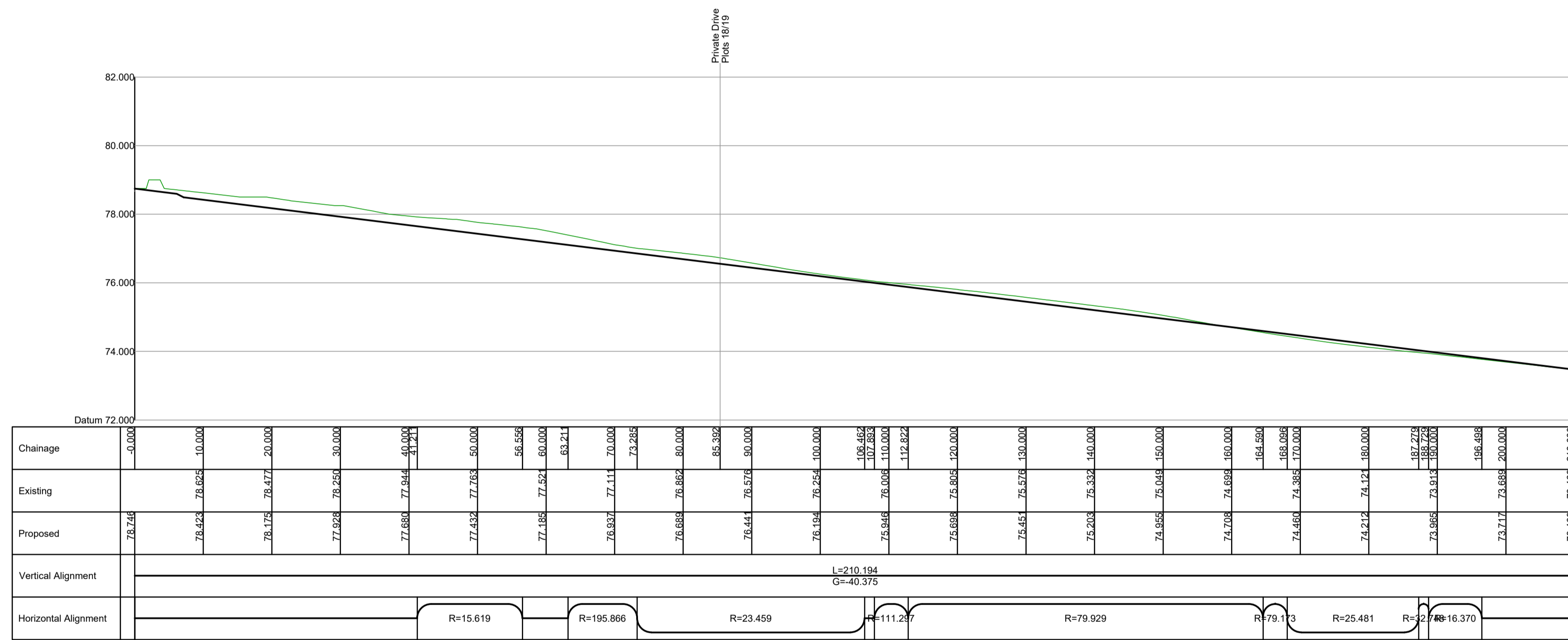
Longitudinal Section Along Main Road Scale 1:500 Horizontal 1:100 Vertical
